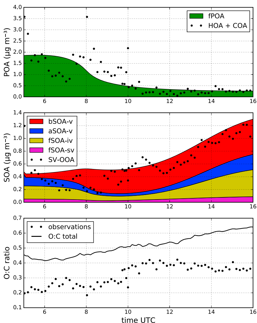
Figure 8. (top) Observed HOA + COA and modeled POA from fuel combustion and cooking (fPOA), (middle) observed SV-OOA and modeled SOA from fuel combustion and cooking (fSOA-sv and fSOA-iv), SOA from anthropogenic VOCs (aSOA-v), and SOA from biogenic VOCs (bSOA-v), and (bottom) observed and modeled O:C ratio evolution, based on the EXP_GRI09_SOARL experiment (Table 2).
