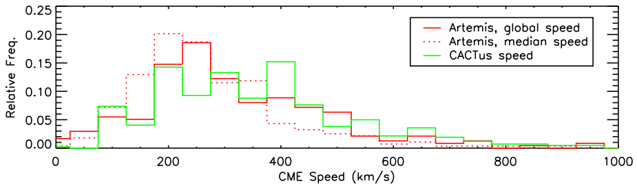
Fig. 76 Comparison of the distributions of speeds of CMEs associated with a SDO/AIA filament eruption: ARTEMIS global (red) and median (dotted red histogram) and CACTus (green)
