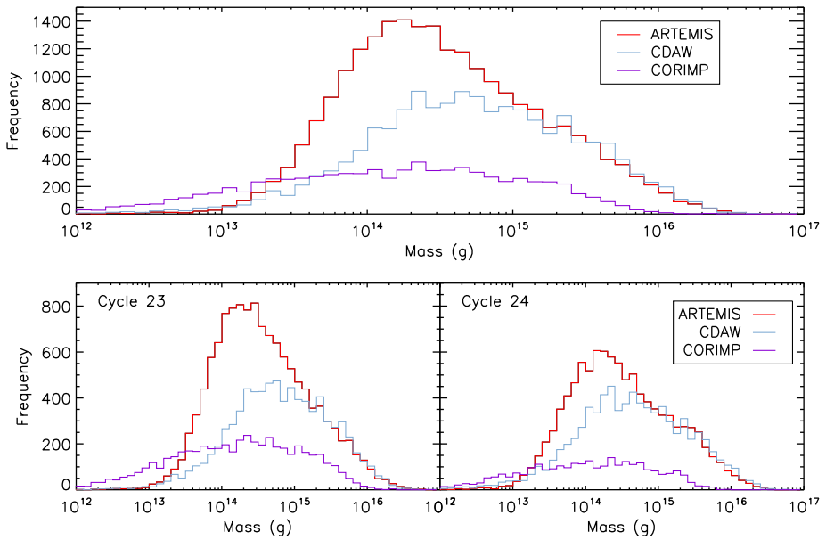
Fig. 12 Histograms of the CME mass distribution from the ARTEMIS, CDAW, and CORIMP catalogs using a log-lin representation. The upper panel covers the two solar cycles and the lower two panels correspond to SC 23 (left) and SC 24 (right)
