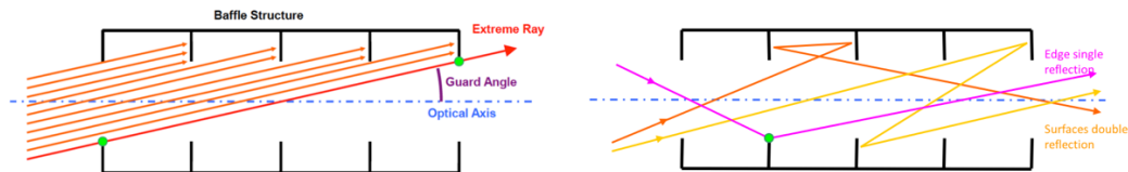
Figure 4: Illustration of the geometrical properties of the entrance baffle: rejection angle and minimum number of reflections on surfaces and edges.
