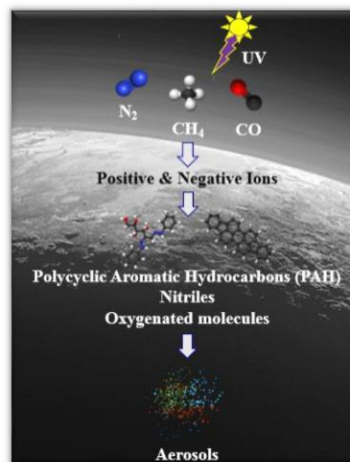
Figure 1: Simplified scheme of Pluto's aerosols formation. Credit (background image): NASA/JHUAPL/SwRI
