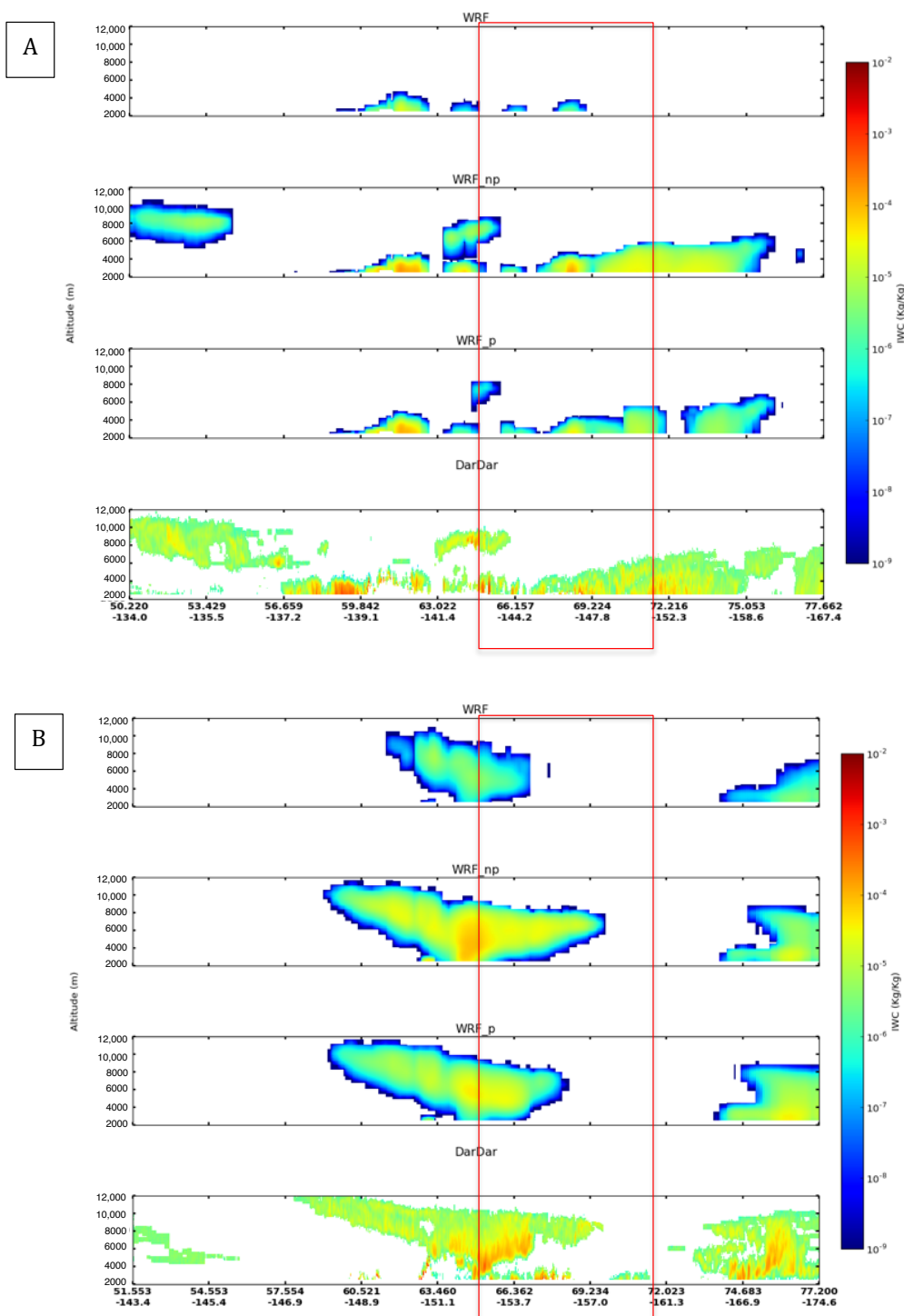
Figure 6. Observed DARDAR and simulated cross section of the ice water content IWC from WRF, WRF_np, WRF_p simulations along T21 (A) and T29 (B) tracks. The red rectangles correspond to the whole area where the flights have been performed (Figure 1).
