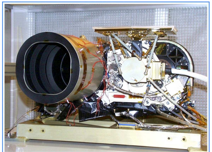
Fig. 5. Flight model of OSIRIS-NAC.
