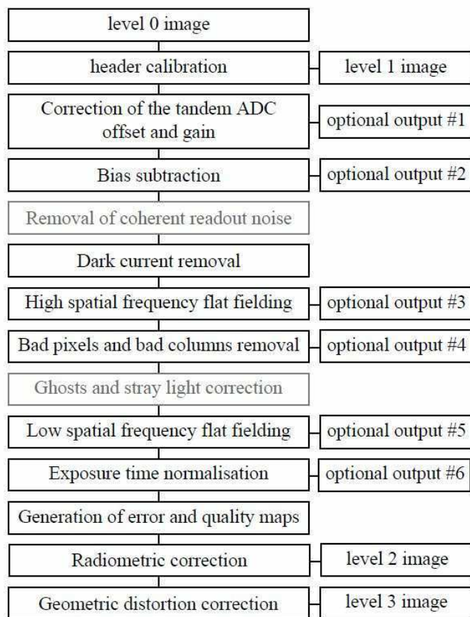
Fig. 6. Flowchart of the OSIRIS calibration pipeline (reproduced from Fig. 2 of Tubiana et al. (2015)).
