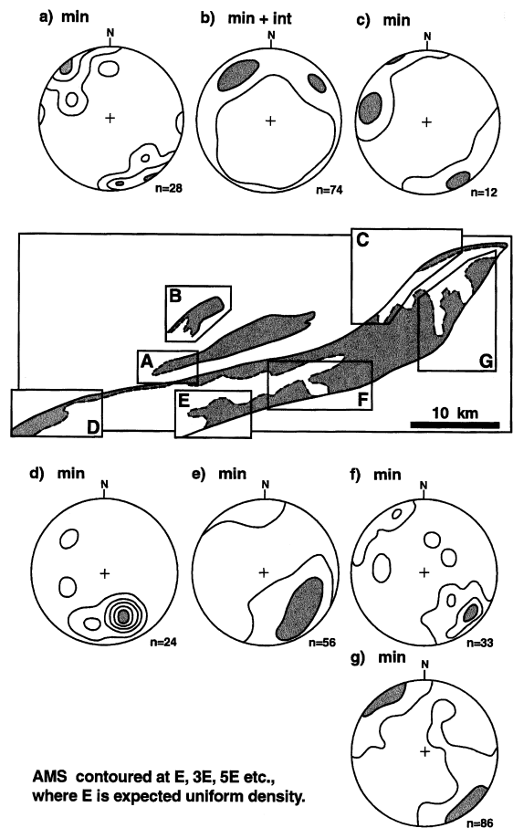
Fig. 4. Orientations of minimum susceptibility (and intermediate where the magnetic fabric is constricted, L > S ) for the anorthosites in seven subareas. Throughout the anorthosites a magnetic foliation trending NE–SW is discernible, to which the pole concentration of minima is orthogonal. The exception is subarea B where fabrics are constricted causing a horizontal girdle of minimum susceptibility axes, defining a vertical magnetic fabric lineation.
