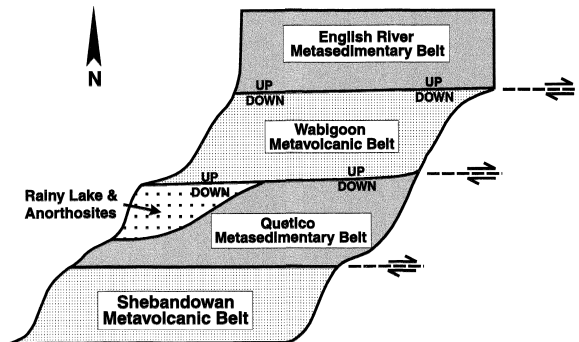
Fig. 14. Schematic map shows the sense of terrain-boundary shear and the senses of vertical motion on the boundaries. Magnetic fabrics confirm this kinematic pattern for the eastern part of the Shebandowan Belt (Borradaile and Spark, 1991; Borradaile and Dehls, 1993) and for the southern margin of the English River Belt (Borradaile et al., 1993a,b). Structural mapping supports dextral transpression of the margins of the Quetico Belt elsewhere (Hudleston, 1976; Borradaile, 1988; Hudleston et al., 1988).
