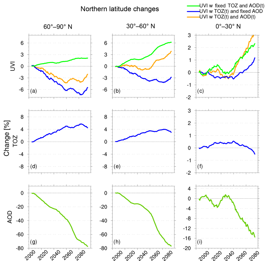
Figure 8. UVI, TOZ and AOD percent change from 2000 to 2010 values in the northern high, middle and low latitudes for the EXP3 experiment. UVI modelled with transient TOZ and AOD fixed at present-day climatological values are in blue. UVI modelled with TOZ fixed at present-day climatological values and AOD variable through the 21st century are in green. UVI modelled with transient TOZ and AOD are in orange. TOZ and AOD are respectively in blue and green.
