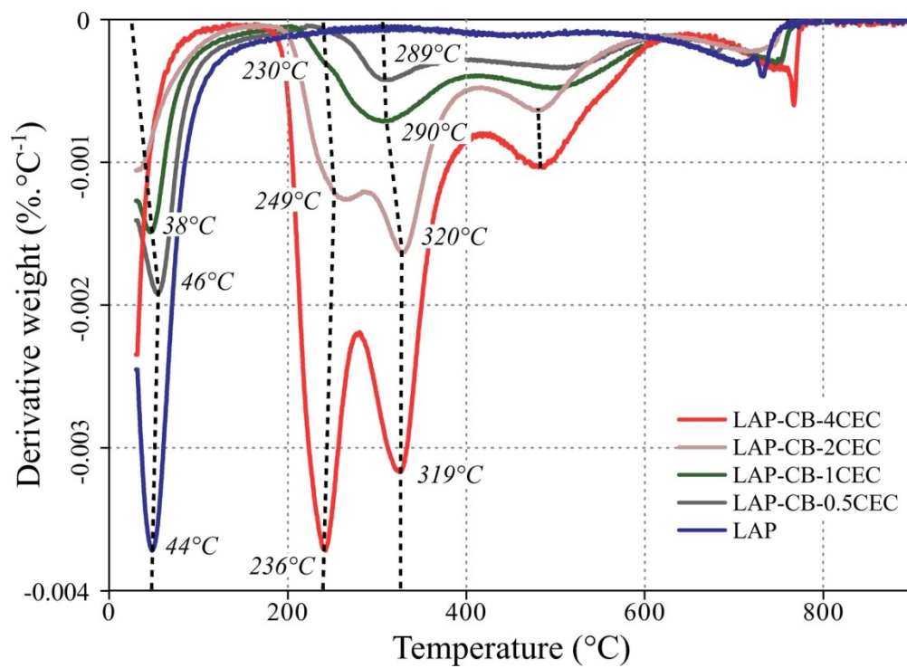
Figure 2: DTG curves for LAP and LAP-CBs between 0 and 900°C with a heating rate of 2°C.min -1
