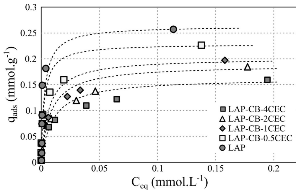
Figure 8: Single-solute adsorption isotherms of Sr 2+ onto LAP and LAP-CBs, dashed dark lines represent the Langmuir fits
