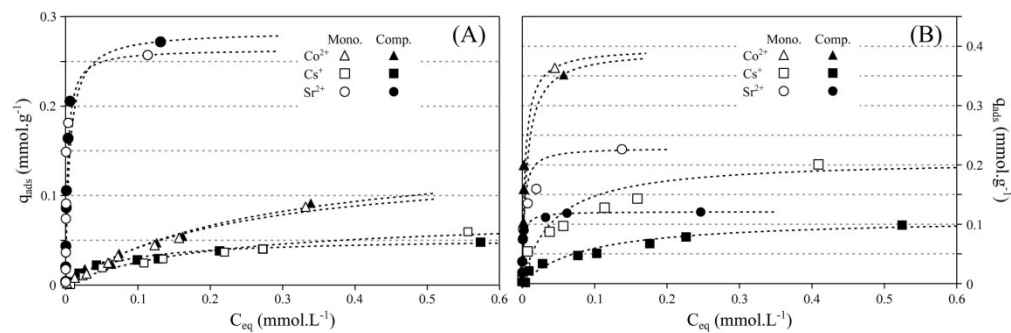
Figure 9: Adsorption isotherms of Co 2+ (triangles), Cs + (squares) and Sr 2+ (circles) in single-solute (open symbols) and competitive (closed symbols) solutions on LAP (A) and LAP-CB-0.5CEC (B). Dashed dark lines represent the Langmuir fits.
