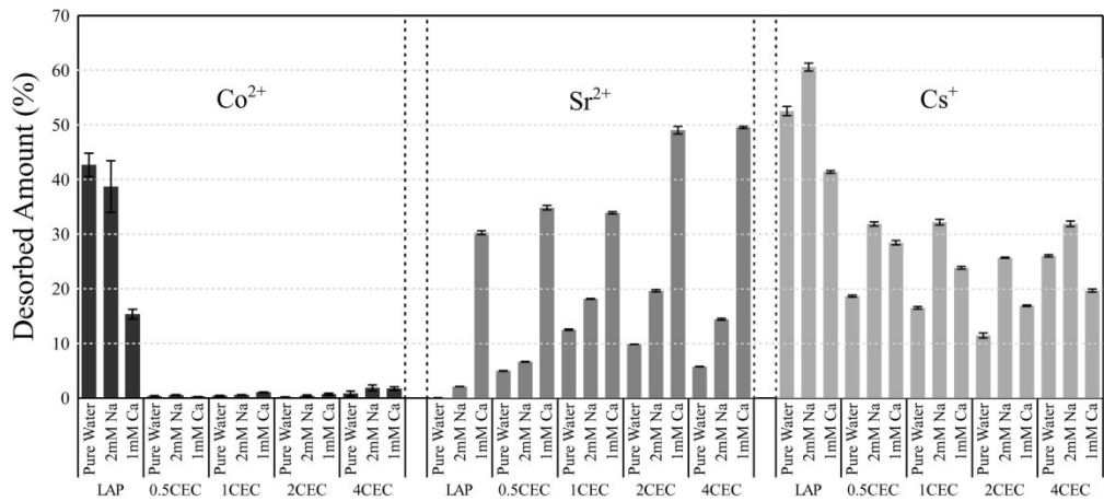
Figure 10: Desorption percentage of Co 2+ (dark rods), Sr 2+ (gray rods) and Cs + (light gray rods) as a function of the adsorbent and the release solutions.
