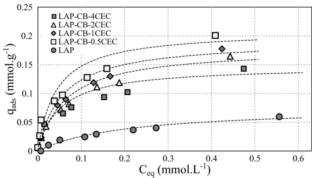
Figure 6: Single-solute adsorption isotherms of Cs+ onto LAP and LAP-CBs, dashed dark lines represent the Langmuir fits
