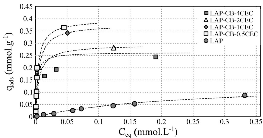
Figure 7: Single-solute adsorption isotherms of \text{Co}^{2+} onto LAP and LAP-CBs, dashed dark lines represent the Langmuir fits
