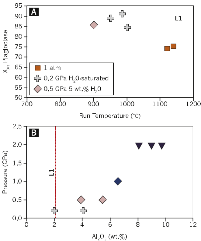
Fig. 5. (a) Variation in molecular An_x in experimentally produced plagioclase from L1 as a function of temperature. The bulk composition of plagioclase phenocrysts from L1 is shown in pink for comparison. The experimental data are from Table 3 (Online only) and the phenocryst composition from Ewart et al. (1973). (b) Al_2O_3 versus pressure of synthesis for augite experimentally crystallised from the basaltic andesite L1.
