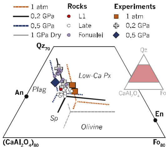
Fig. 6. Bulk rock compositions for Late and Fonualei projected within the pseudo-ternary CaAl_2O_4 -silica-forsterite system using the scheme of O'Hara (1968). Plotted for comparison are cotectics for plagioclase and pyroxenes at 1 atm, 0.2 GPa ( H_2O -saturated), and 0.5 GPa (with 5 wt% of H_2O in the liquid phase). The plagioclase-pyroxene cotectics are based on experimental data from this study (Table 3 – Online Only). The natural rock compositions are from Ewart et al. (1973), Caulfield et al. (2012), Turner et al. (2012) and Beier et al. (2017).
