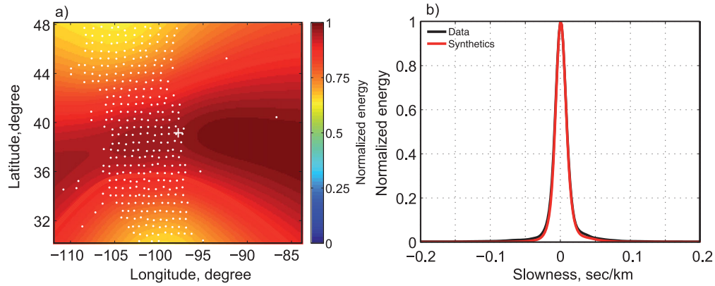
Figure A2. Results of the beamforming for the phase PKIKP . (a) Energy B_R integrated in the slowness interval \delta s = [-0.01, 0.01] \text{ s km}^{-1} . The observations are represented as a colourmap and the synthetics with coloured lines. The energy is normalized for the synthetics and data separately for an easier comparison. The locations of the stations are represented with the black points. (b) The energy B_s , computed over the all area since no focusing is observed.
