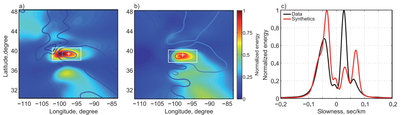
Figure 12. Results of the beamforming for the phases SKKS . (a) Energy B_R for the waves propagating along the minor arc and integrated in the slowness interval \delta s = [0.02 \ 0.05] \text{ s km}^{-1} for the observations and synthetics. The observations are represented as a colourmap and the synthetics with coloured lines. The energy is normalized for the synthetics and the data separately for an easier comparison. (b) Energy B_R for the waves propagating along the major arc ( \delta s = [-0.05 \ -0.02] \text{ s km}^{-1} for the observations and synthetics). (c) Energy B_s around main focusing locations \delta x \delta y (shown with the grey rectangles in a, b).
