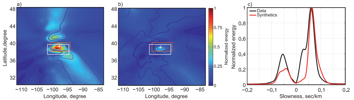
Figure 11. Results of the beamforming for the phases PPS . (a) Energy B_R for the waves propagating along the minor arc and integrated in the slowness interval \delta s = [0.045 \ 0.075] \text{ s km}^{-1} for the observations and \delta s = [0.05 \ 0.08] \text{ s km}^{-1} for the synthetics. The observations are represented as a colourmap and the synthetics with coloured lines. The energy is normalized for the synthetics and the data separately for an easier comparison. (b) Energy B_R for the waves propagating along the major arc ( \delta s = [-0.075 \ -0.045] \text{ s km}^{-1} for the observations and \delta s = [-0.08 \ -0.05] \text{ s km}^{-1} for the synthetics). (c) Energy B_s around main focusing locations \delta x \delta y (shown with the grey rectangles for the observations and orange rectangles for the synthetics in a, b).
