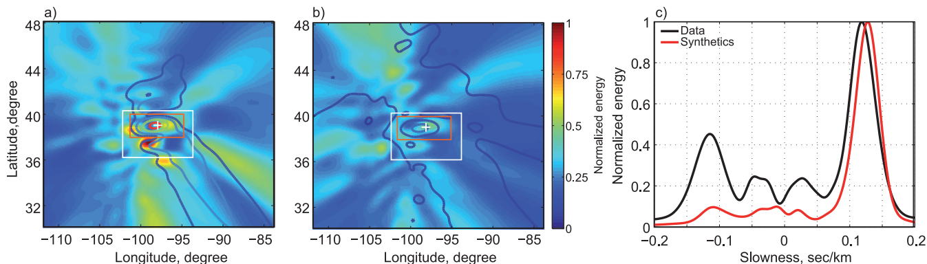
Figure 13. Results of the beamforming for the phases SSS. (a) Energy B_R for the waves propagating along the minor arc and integrated in the slowness interval \delta s = [0.095 \ 0.145] \text{ s km}^{-1} for the observations and \delta s = [0.105 \ 0.15] \text{ s km}^{-1} for the synthetics. The energy is normalized for the synthetics and data separately for an easier comparison. (b) Energy B_R for the waves propagating along the major arc ( \delta s = [-0.145 \ -0.095] \text{ s km}^{-1} for the observations and \delta s = [-0.15 \ -0.105] \text{ s km}^{-1} for the synthetics). (c) Energy around main focusing locations \delta x \delta y (shown with the grey rectangles for the observations and orange rectangles for the synthetics in a, b).
