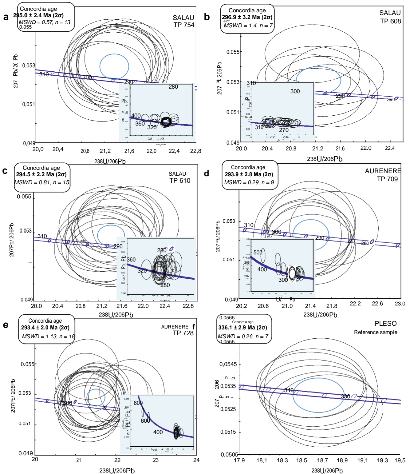
Fig. 9 Tera-Wasserburg concordia diagrams for zircon. a–b–c Salau granodiorite. d, e Aurenere granodiorite. f Pleso reference sample. N corresponds to the number of zircon grains that have been analyzed per sample. Ellipses and errors are reported at 2\sigma
