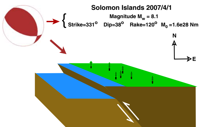
Fig. 1 Solution obtained for a Solomon Island Earthquake. The “beach ball” is the standard graphical representation of the moment tensor. The angles define the fault plane associated to the best double-couple. Here the fault plane is identified by the tectonic setting (subduction zone)
