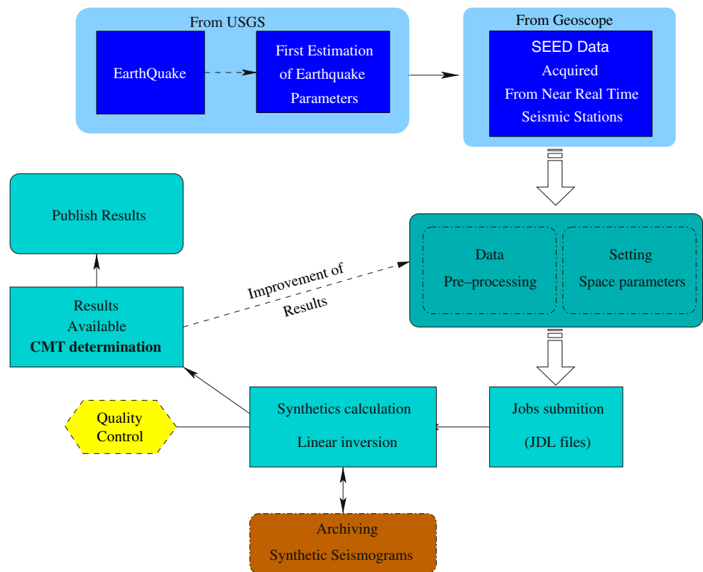
Fig. 3 Work flow used for the determination of the seismic moment tensor at the centroid of an earthquake
