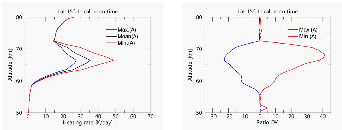
Figure 13. Calculated solar heating rate profiles for the observed maximum, minimum, and mean albedo at local noon time at 15°S. The solar heating rate is displayed in \text{K day}^{-1} (left) and as a relative ratio from the mean albedo (right).
