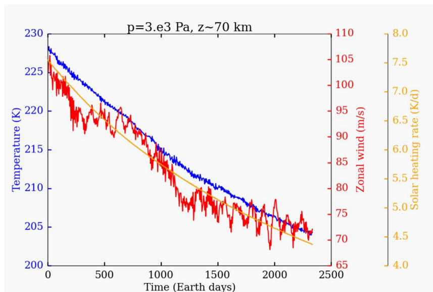
Figure 14. Temporal variations of zonal mean solar heating rate (orange), wind speed (red), and temperature (blue) at 10°S–20°S at 30 mbar ( \sim 70 km). The solar heating rate is controlled to decrease smoothly along time by 40% from the reference condition in the IPSL Venus GCM (Appendix). Simultaneous variations in temperature and zonal wind speed are shown together.
