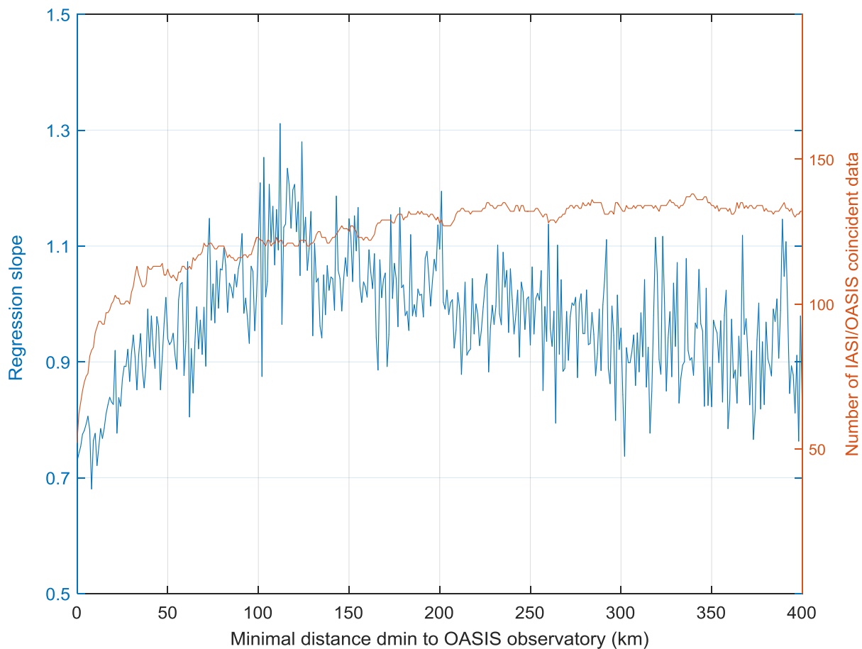
5 Figure 7: Regression slope (blue lines, left axis) between IASI and ground-based FTIR observations with temporal sampling difference smaller than 30 min, as a function of d_{min} to OASIS observatory, considered for the calculation of the 15 km wide rings. The data (orange lines, right axis) show the total number of IASI/OASIS coincident observations.
