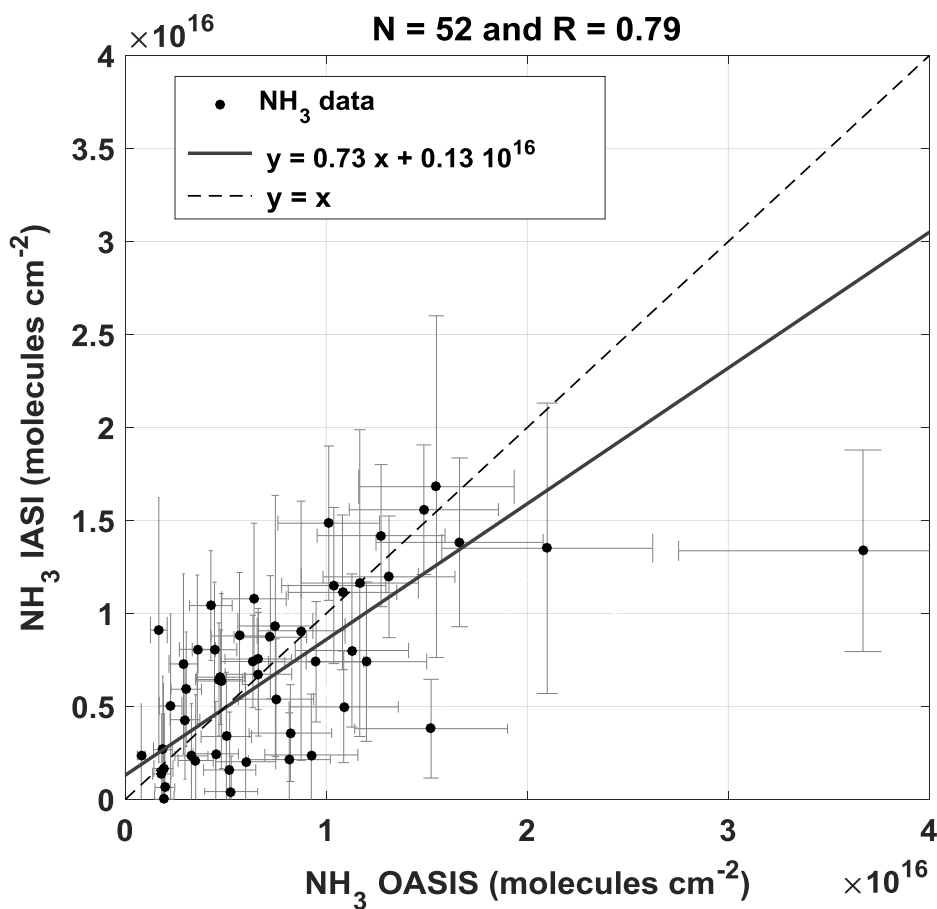
Figure 4: Correlations between the FTIR/OASIS and IASI \text{NH}_3 total columns fulfilling the temporal and spatial coincidence criteria: a time difference smaller than 30 min, and a 15 km radius centered on the ground-based FTIR station. The dashed line is the straight equation with slope 1.
