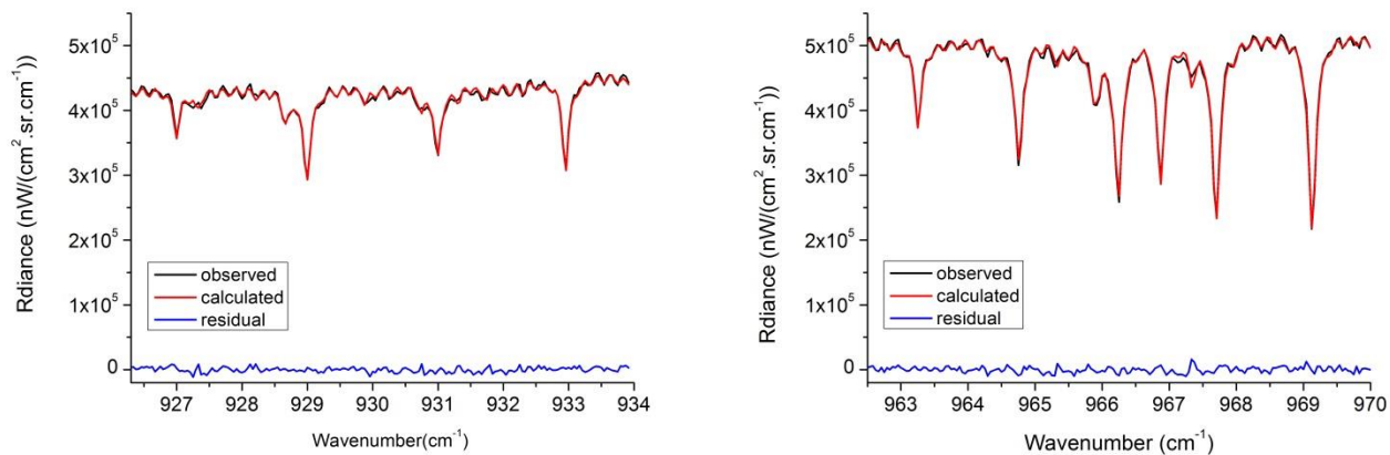
5 Figure 3: Observed (black line) and calculated spectrum (red line) in radiance unit ( \text{nW}/(\text{cm}^2.\text{sr}.\text{cm}^{-1}) ) for both spectral windows measured with the BRUKER Vertex 80 in Creteil on the 21st March 2012 with the fitting residuals (blue line).
