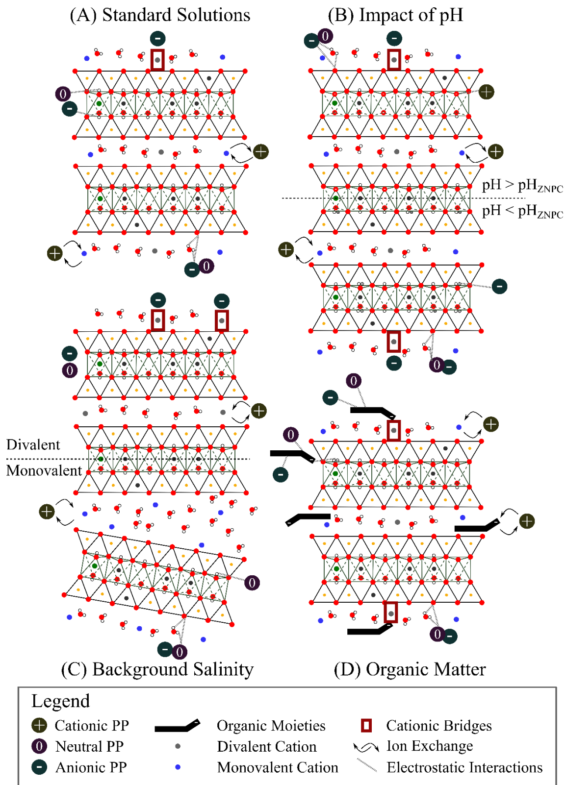
Figure 5. Schematic representation of the impact of the enrichment of the solution from standard solution (A), to impacts of pH (B), background salinity (C) and organic matter (D) on the adsorption mechanisms of PPs for different charge states
