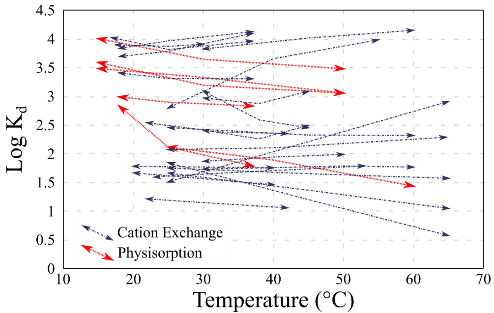
Figure 3. Impact of the temperature on the variation of the solid/water partition (Log K_d ) of PP onto adsorbent as a function of the sorption mechanisms, with cation exchange (blue dashed lines) and physisorption (red dashed lines), raw data and references are available in Table 7.
