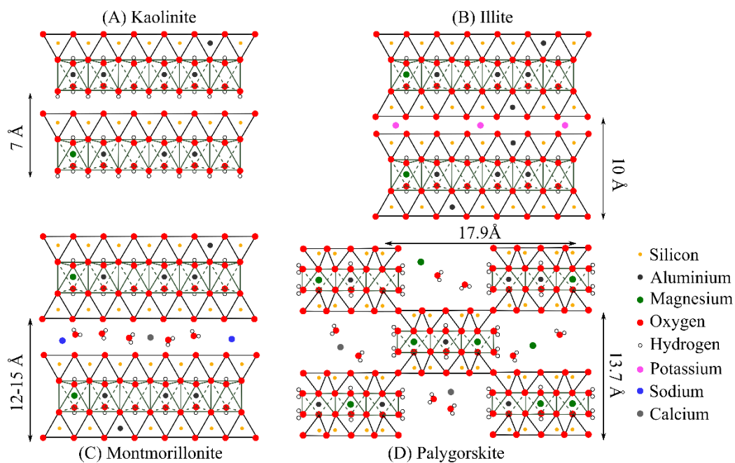
Figure 1. Examples of different layer structures of clay minerals with (A), kaolinite (1:1), (B), illite (non-expanded 2:1), (C), smectite (expanded 2:1) and (D), palygorskite (fibrous 2:1).
