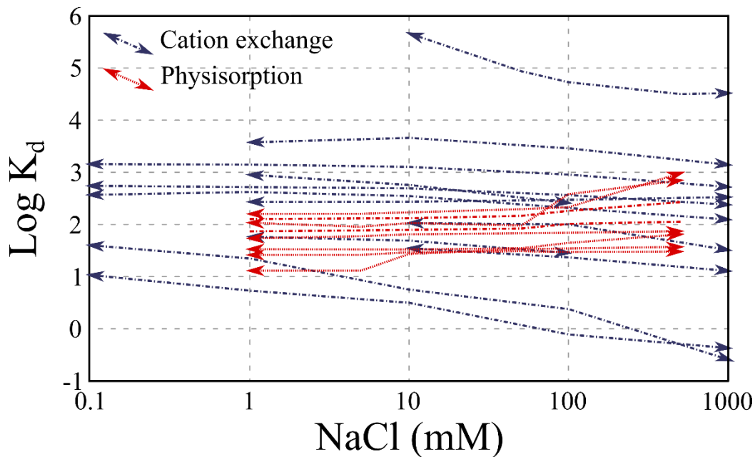
Figure 4. Impact of NaCl concentration (in mM) on the solid/water partition of PP (Log K_d ) onto adsorbent as a function of the adsorption mechanism with cation exchange (blue dashed lines) and physisorption (red dashed lines), raw data and linked references are available in Table 8.
