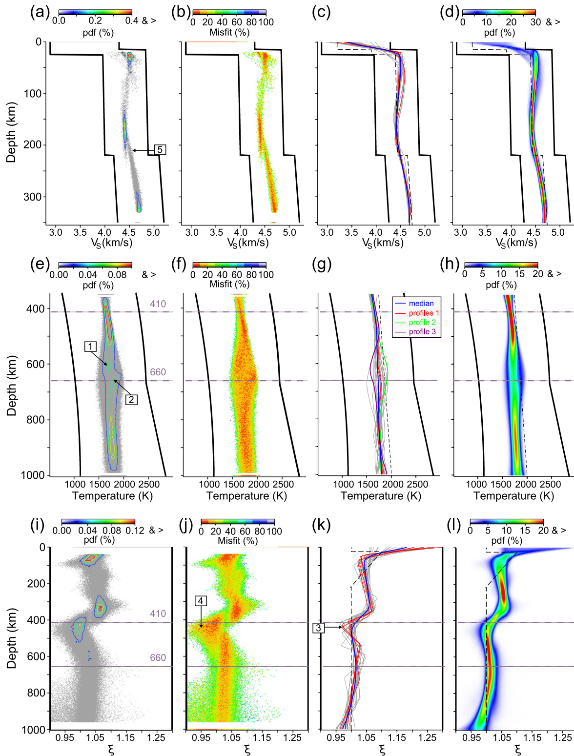
Figure 8. Same as Fig. 4 but for the Vanuatu–California data. Dashed lines in (c), (d), (k) and (l) are PREM values. Dashed lines in (g) and (h) show the 1600 K adiabat considering a temperature gradient of 0.4 \text{ K km}^{-1} . Blue lines in (c), (g) and (k) are the median profiles of the distributions.
