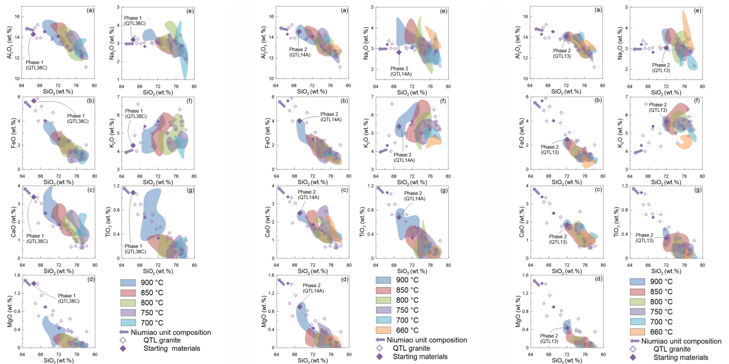
Figure 10. (middle two columns) Whole-rock compositions of the Qitianling granites ( \diamond ) and starting materials ( \blacklozenge ) (totals normalized to 100 wt %) compared to residual glass compositions from the Phase 1 (QTL38C, left two columns) and the Phase 2 (QTL14A, middle two columns and QTL13, right two columns) experiments (QTL38C). The Niumiao unit compositions are from Feng et al. (2012).
