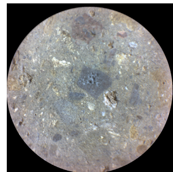
Fig. 1: Example SuperCam RMI of a rock with LIBS analysis pits ( \sim 350\text{ }\mu\text{m} diameter) on the central dark gray grain. The distance is 2 m and the image is corrected for flat field, contrast, balance, and color.
