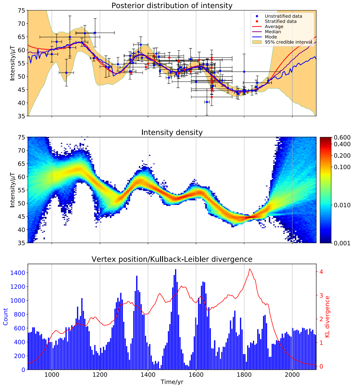
Figure 15. The posterior intensity variation for the Lübeck-Paris700 data set. Top panel: the average, median and modal curves with 95 percent credible intervals shown in orange. Middle panel: density plot of the posterior distribution. Bottom panel: combined plot of a histogram of the vertex position showing the most likely ages for change in linear slope, with the KL divergence in red (right-axis).
