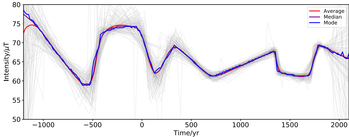
Figure 7. An ensemble of 1000 individual models (equally spaced along the Markov chain) in grey, compared to the ensemble statistics, for the AH-RJMCMC method applied to the Synt-Paris700 data set.
