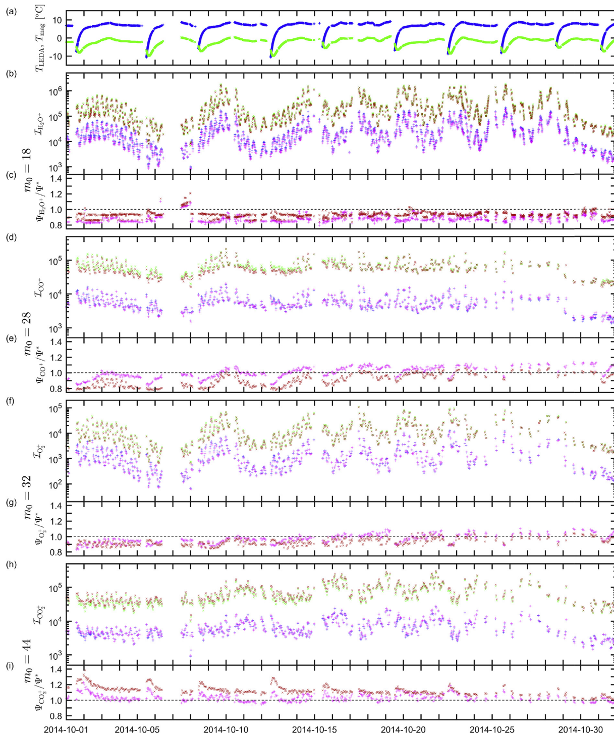
Fig. 7. Ion count rates for October 2014. (a) LEDA and magnet temperature in blue and green respectively, Ion count rates are given for (b–c) \text{H}_2\text{O}^+ , (d–e) \text{CO}^+ , (f–g) \text{O}_2^+ and (h–i) \text{CO}_2^+ . Count rates for channel A are indicated with + symbols, in blue for the count rates based on peak height, magenta for the count rates based on peak area; count rates for channel B are indicated with × symbols, in green and red for count rates based on peak height and area, respectively. The count rates for channel B have been multiplied by 10 to improve figure readability. The ratio of both count rates, \Psi/\Psi^* , varies with instrument temperature; while it is rather constant for \text{H}_2\text{O}^+ , it tends to increase at low temperature for \text{CO}_2^+ but decreases for \text{CO}^+ and \text{O}_2^+ . (For interpretation of the references to colour in this figure legend, the reader is referred to the Web version of this article.)
