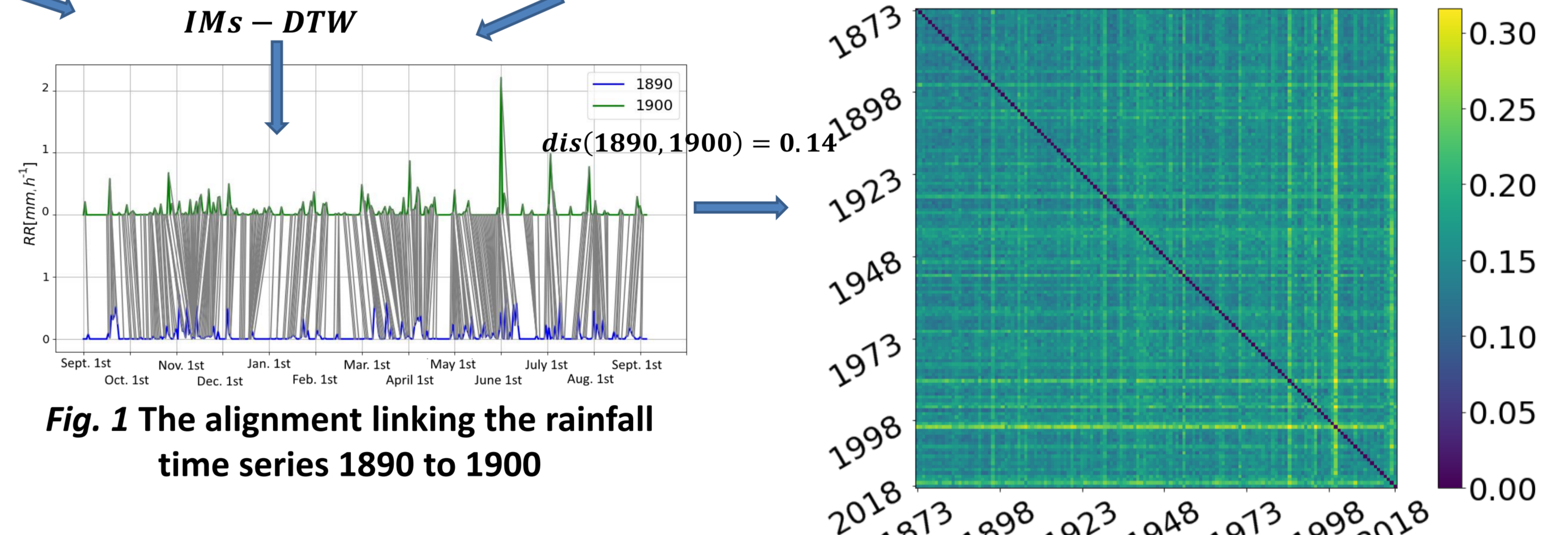
Fig. the dissimilarity matrix D (146x146) between the 146 annual time series measured in Paris-Montsouris between 1873 and 2019
