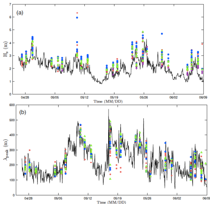
Figure 23: Time series of (a) H_s in m (b) peak wavelength in m from SWIM and from the OSSI probe in Moorea ( -149.82^\circ\text{E} , -17.61^\circ\text{N} ) between April 28 th 2019 and June 9 th 2019. The black curve indicates the in situ measurements. The CFOSAT nadir measurements are reported in magenta in panel a. The CFOSAT 6, 8 and 10^\circ beams are reported in red, blue and green (panels a and b).
