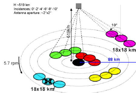
Figure 1 SWIM beam rotation and incidence angles
