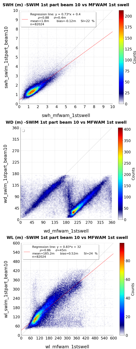
Figure 19: Same as Fig.18, but for the parameters of the 1 st partition if the SWIM spectra (beam 10°) compared to the parameters of the 1 st swell of MFWAM
