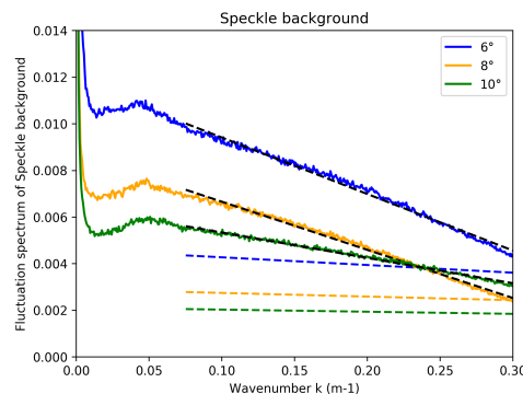
Figure 14: Mean background density spectra as a function of wave number (rad/m) for beams 6^\circ (solid blue), 8^\circ (solid orange) and 10^\circ (solid green). Dashed black lines correspond to the triangle-shaped model fitted on these spectra (adjustment between k=0.075 and 0.3 rad \text{m}^{-1} ). Dashed colored lines correspond to Eq.2 with the theoretical values of N_{\text{ind}} and \delta r . This figure corresponds to data selected over a 7-day period (26 April-1 May 2019) in the [-10^\circ, 10^\circ] latitude range and for surface conditions with H_s less than 2 m and wind speed less than 5 m/s).
