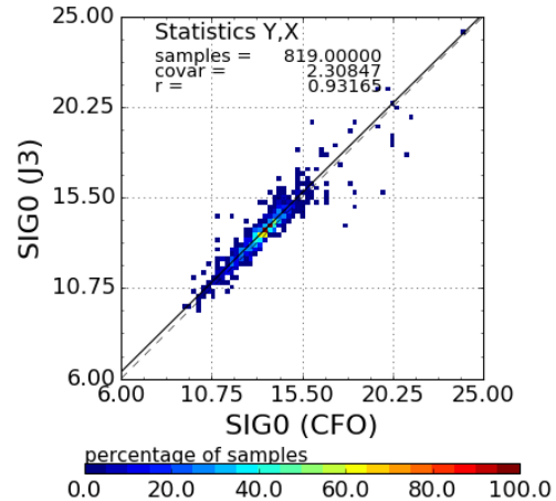
Figure 8: Same as Fig.7 but for the nadir \sigma_0 values.
