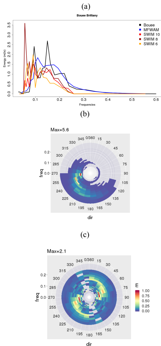
Figure 22: Same as Fig. 21 but for a case on July 24 th 2019, 18:00UTC
