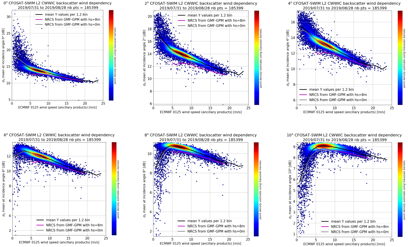
Figure 11: Distribution of \sigma_0 values at 0, 2, 4, 6, 8 and 10^\circ (\pm 0.5^\circ) as a function of wind speed (taken from the ECMWF model). The black line shows the mean value. The color lines correspond to mean values of GPM data for the same wind and for significant wave heights of 0m (green) and 8m (purple)
