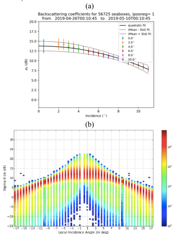
Figure 10: (a) SWIM mean profiles of \sigma_0 with incidence angle over the free ocean surface; (b) statistics of \sigma_0 from GPM/PR data for negative and positive incidence angles with respect to nadir (N. Longepe, personal communication).
