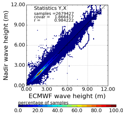
Figure 5: Significant wave height from SWIM nadir observations compared to ECMWF model data for a 13-day period (9-21 September 2019).
