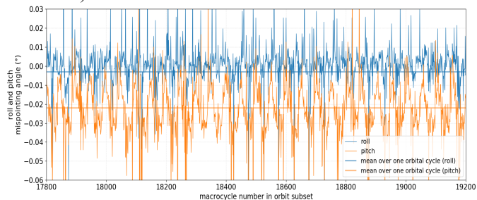
Figure 4: Zoom of roll (blue curve) and pitch (orange curve) mispointing angles estimated in the level 1A processing over about 5 minutes. The thick blue and orange horizontal lines show the mean roll and pitch angles, respectively, averaged over one cycle of data (13 days).
