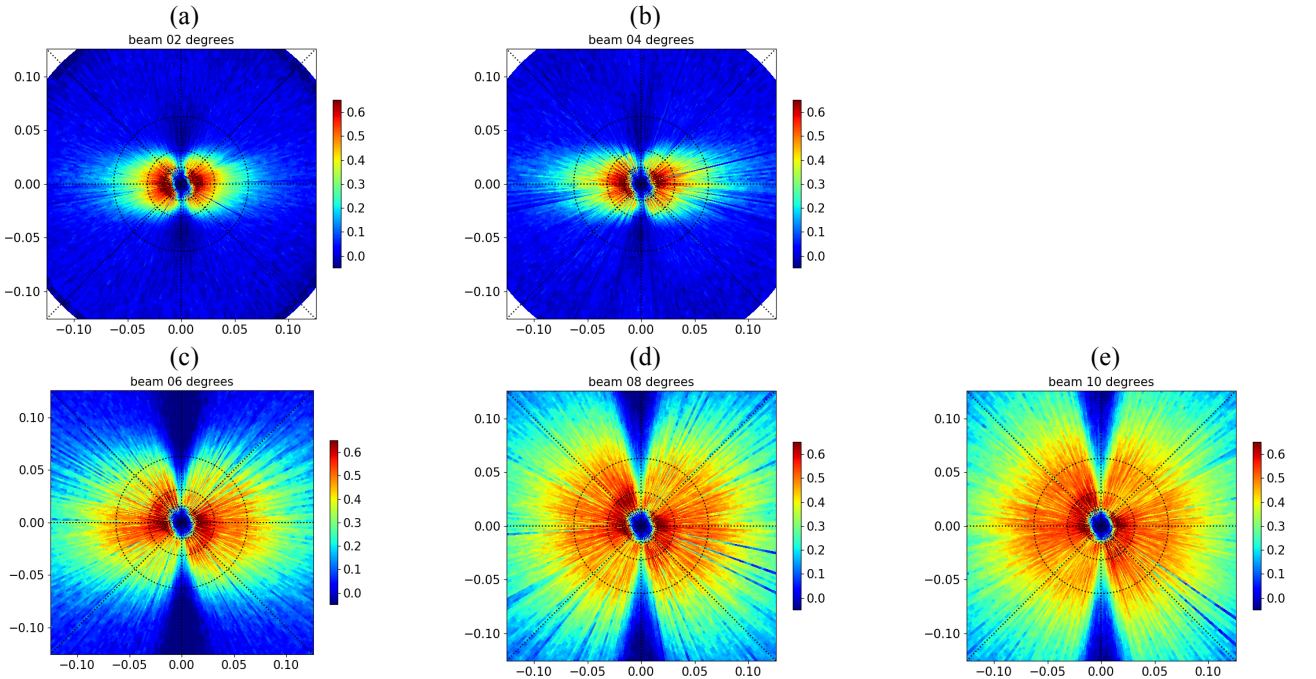
Figure 13: Polar plots of the correlation coefficient between SWIM fluctuation spectra and WW3 collocated wave slope spectra for the data set from April, 25 th to April, 30 th , 2019. Horizontal and vertical axes refer to the wave number of the waves in two orthogonal directions, with the vertical axis aligned with the satellite along-track direction. Panels (a, b, c, d, e): for SWIM beams 2°, 4°, 6°, 8°, 10°, respectively.
