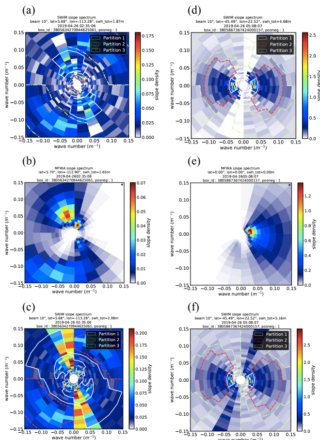
Figure 17: Examples of wave spectra from the 10° beam observations with the speckle correction from the models presented in this paper (a, d) and the original correction (c, f). (b, e) show the corresponding MFWAM wave slope spectra. The horizontal and vertical axes refer to East-West and North-South directions, respectively. The white, red and yellow contours on the SWIM spectra indicate the partitions (see section VIII). Date and position of observations are April 26 th 2019 02:35 UTC at [5.68N,113.27W] for (a-c) and April 26 th 2019 05:08UTC at [45.49S,22.51E] for (d-f)
