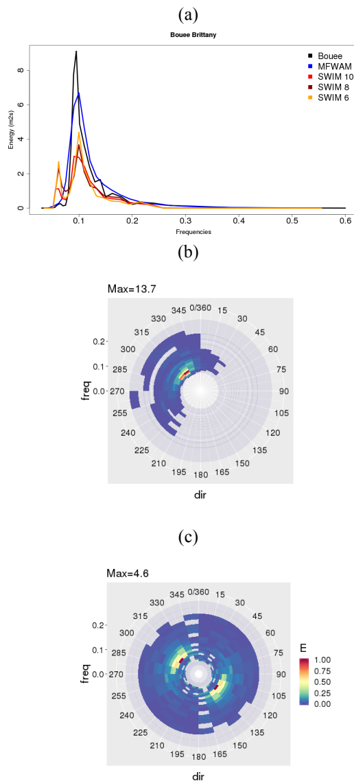
Figure 21(a) Omni-direction spectra (m 2 /s) from the Brittany buoy (47°33’0” N 8°28’12” W), MFWAM and SWIM (3 beams with the red, brown and yellow curve as indicated in the insert) on August 19 th 2019 18:00 UTC. (b, c) directional spectrum from (b) the buoy, (c) SWIM beam 10°. In (b, c), the color scale is relative to the maximum of energy of each plot.
