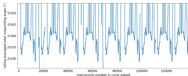
Figure 3: Rolling average of the total mispointing angles estimated in the level 1A processing over several orbits of 1.5h each, with respect to macrocycle number in the selected subset. Values are averaged over 500 macrocycles. The oscillations show the impact of the reference ellipsoid.
