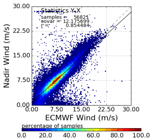
Figure 9: SWIM nadir wind speed compared to ECMWF wind speed for a 13-day period (9-21 September 2019)
