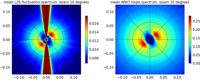
Figure 12: Mean fluctuation spectra for the period from April 25 th to April 30 th 2019 (left) compared to the mean wave slope spectrum obtained from collocated points of WW3 outputs (right). Horizontal and vertical axes refer to the wave number of the waves in two orthogonal directions, with the vertical axis aligned with the satellite along-track direction.
