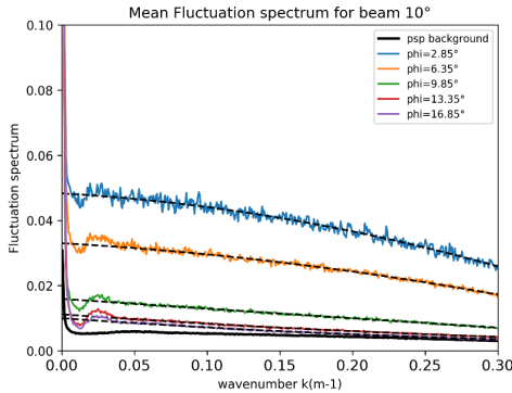
Figure 15: Color lines: Mean fluctuation spectra for the SWIM beam 10°, obtained by accumulating data over different azimuthal angles (from about 2 to about 17°, w.r.t. the along-track direction, see insert legend) and over 6 days of observations (26 th April - 1 st May 2019). The dashed black lines represent the polynomial fit (estimated for k within [0.075 to 0.3] rad/m). The solid black line is the mean background speckle spectrum. See text for details.
