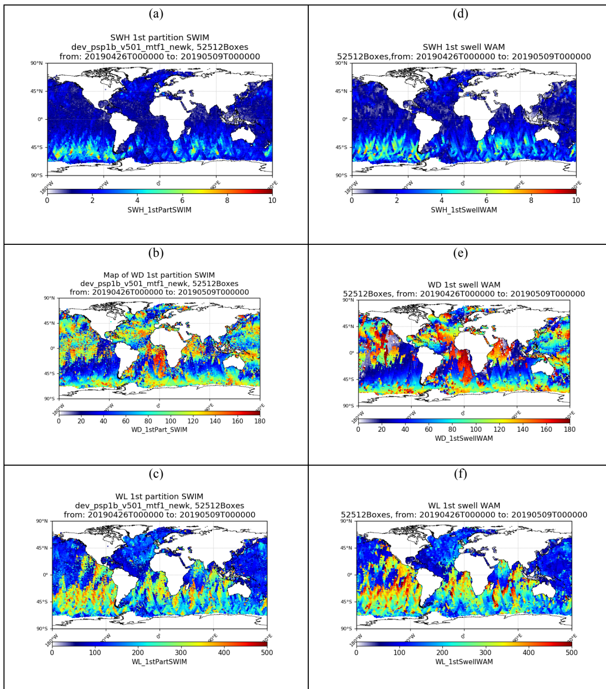
Figure 20 : Maps of SWIM (a, b, c) and MFWAM (d, e, f) parameters for a period of about 13 days starting on April 26 th 2019 02 :00. a and d: wave height of the first partition; b and e: direction of the first partition (for MFWAM the directions have been folded in the [0-180°] interval to be compared with the SWIM data); c and f: wavelength of the first partition. The SWIM results are shown for the 10° incidence beam. See text for details.
