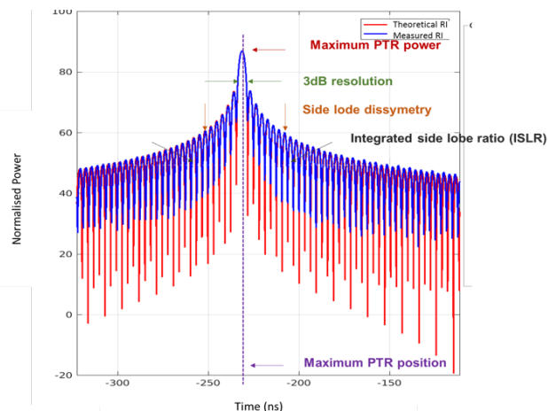
Figure 2: Point Target Response (PTR). Blue line: measured, red line: theoretical sinus cardinal function.
