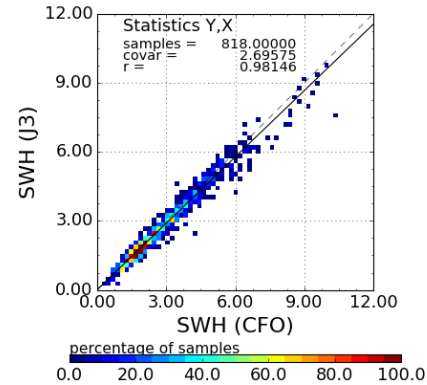
Figure 7: Significant wave height from SWIM nadir observations compared to Jason 3 altimeter values at crossover points for time difference less than 3h (1 orbital cycle: 14-26 August 2019)
