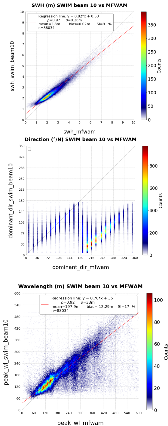
Figure 18: Scatter plots of SWIM parameters from the 10° beam full spectra as a function of MFWAM full spectra parameters, for a 13 days period (26 April-8 May 2019)- (a) Significant wave height Hs; (b) Dominant direction (from North; (c) Dominant wavelength. The color code represents the number of points per bin of values. The red line on (a) and (c) represents the linear fit.
