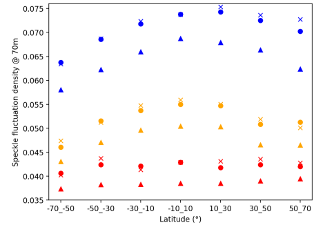
Figure 16: Speckle noise spectral level at k = 0.09 rad/m (wavelength of \sim 70 m), calculated from our empirical formulation, at the azimuth angle of maximum speckle level ( \phi = \phi_0 ). The results are plotted for the three SWIM beams in blue (6°), orange (8°), red (10°) and for three sea surface conditions (circle: H_s < 2m & U < 5m/s , cross: H_s < 2m & 5 < U < 9m/s , triangle: 2m < H_s < 4m & 5 < U < 9m/s ).
