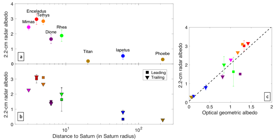
Figure 1. (a) Averaged 2.2-cm disk-integrated radar albedos of Saturn’s major satellites. The error bars show the dispersion of the data set for each satellite. The statistical uncertainties on the derived albedos (inferred from the goodness of the fit; supporting information) are smaller than the size of the symbols. (b) Average 2.2-cm disk-integrated radar albedos measured on the leading and trailing hemispheres of each of Saturn’s satellites. Note that the large error bar for Rhea’s leading hemisphere is due to the strong contrast between the radar-bright ejecta blanket of the Inktomi crater and the radar-darker rest of Rhea’s leading side. (c) Optical geometric versus 2.2-cm radar albedos. The optical geometric albedos are from Verbiscer et al. (2007; see also Hendrix et al., 2018) up to Rhea. Those for Iapetus and Phoebe are from Morrison et al. (1986). The best linear fit between these quantities is indicated (black dashed line); it relates the optical geometric albedo p to the 2.2-cm radar albedos A_{SL-2} as follows: A_{SL-2} = 1.98p + 0.07 .
