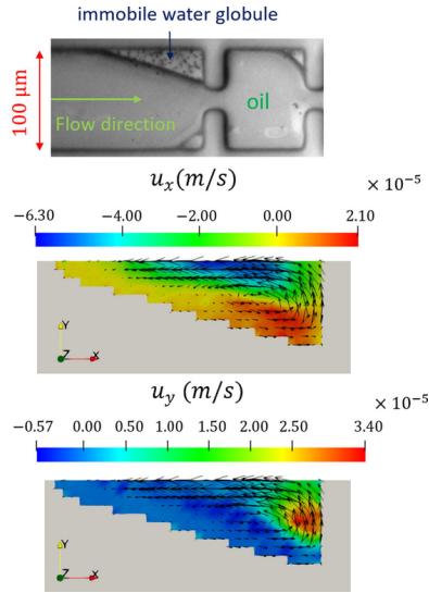
Fig. 2. Immobile pocket of water and velocity fields measured using micro-PIV.
