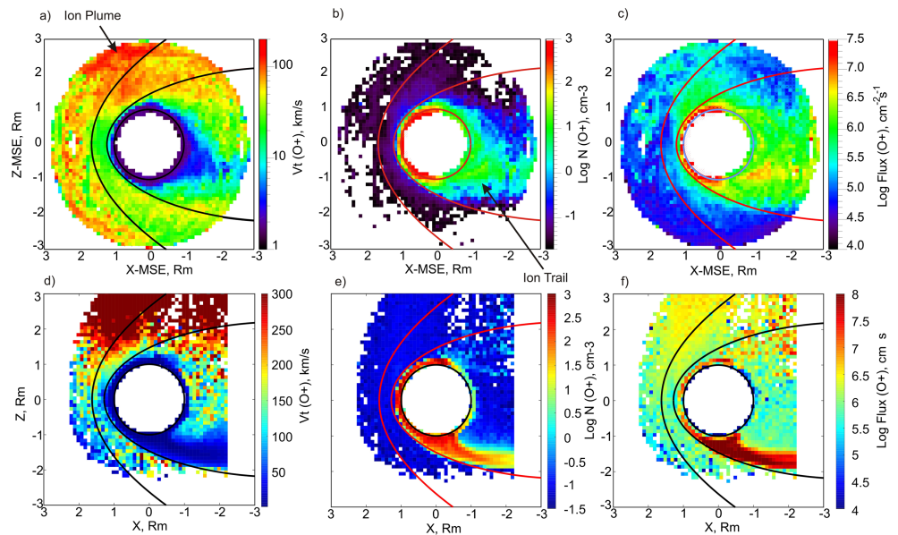
Figure 1. Maps of the O^+ ion velocity (a), density (b), and fluxes (c) plotted in the XZ_{MSE} planes ( -0.5R_M < Y_{MSE} < 0.5R_M ). Black (red) curves show the nominal positions of the bow shock and the magnetospheric boundary (Dubinin et al., 2006). (d–f) Maps of the same values from the simulation run. Ion plume and ion trail are well seen in the observations and simulations. MSE = Mars Solar Electric system.
