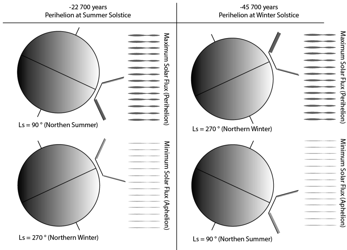
Fig. 8. Insolation received by a north- or south-facing slope located at the equator in two opposite cases. At 45.7 ka, the longitude of perihelion was very similar to the present day ( L_s = 251^\circ ), south-facing slopes
