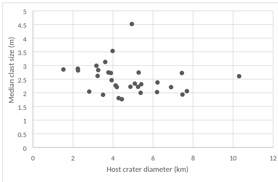
Fig. S2 Median clast size of rockfalls with respect to the host crater diameter
