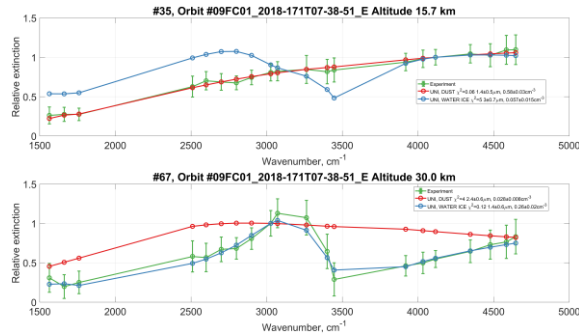
Fig. 1: Results of the fitting procedure. Measured normalized extinction (green line with error bars) and fitted results for water ice particles (blue) and dust particles (red) for orbit #9FC_E (20 June 2018).
