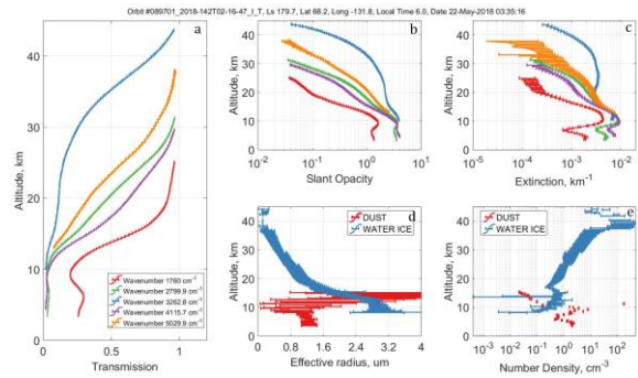
Fig. 2: Retrieved vertical profiles of transmission (a), slant opacity (b), and extinction coefficient (c), particle effective radius (d), and number density (e) from orbit #897_I (22 May 2018).
