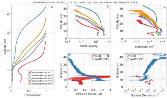
Fig. 2: Retrieved vertical profiles of transmission (a), slant opacity (b), and extinction coefficient (c), particle effective radius (d), and number density (e) from orbit #897_I (22 May 2018).
