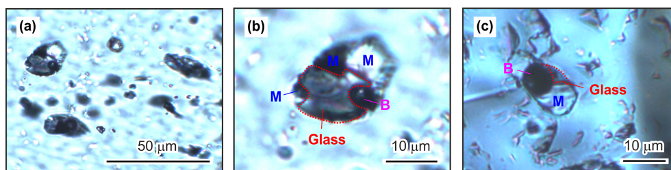
Figure 5. Microphotographs of characteristic melt inclusion textures in olivine (taken in transmitted light with partly crossed polarizer). (a) Many melt inclusions have approximately ellipsoidal, but nevertheless variable shape. (b) Close up of microphotograph in (a) showing that the melt inclusions have abundant microlites (M) and mostly relatively low glass and bubble (B) volumes. (c) Melt inclusion with a bubble that apparently makes up >10 vol%.
