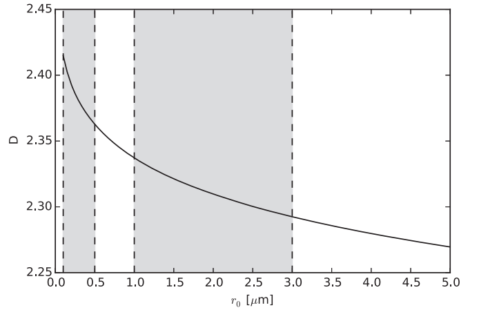
Figure 3. Fractal dimension D as a function of r_0 . The shaded areas denote the range of r_0 measured in comets Wild 2 and Churyumov–Gerasimenko.
