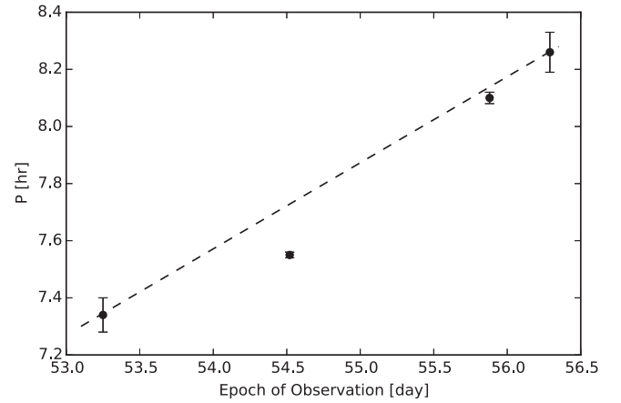
Figure 1. 'Oumuamua’s reported rotation period as a function of epoch of observations (in MJD = JD-2458000.5). The data are as listed in Table 1 and described in the text. The plotted line simply connects the first and last data points, to guide the eye.
