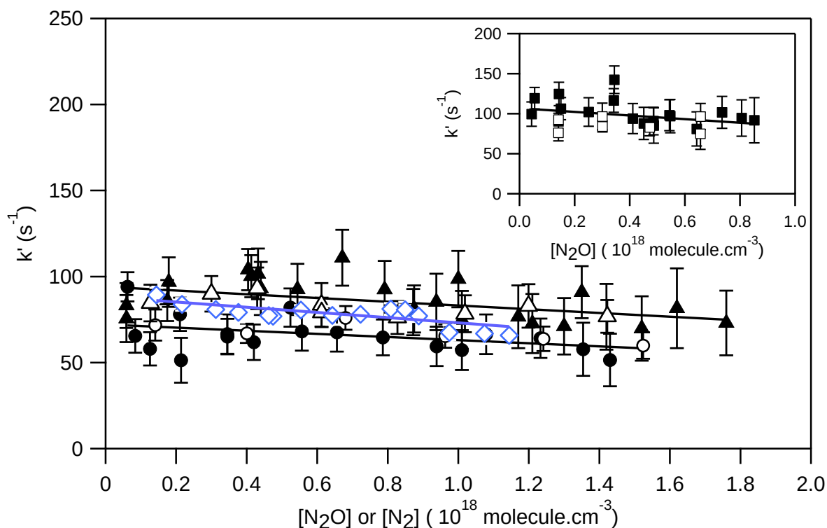
Fig. 1. Pseudo-first order rate coefficients for the loss of OH radicals ( k' ) plotted against the N_2O and N_2 concentrations. The lines represent the linear least-squares fits of data and the slope yields the bimolecular rate coefficient k_1 . The filled symbols were obtained in 99% pure N_2O while the open symbols were from 99.998% pure N_2O at 372 K (■ and □), 298 K (▲ and △), and 253 K (● and ○). The obtained values of k_1 at 372, 298, and 253 K are, respectively, (-2.26 \pm 1.34) \times 10^{-17} , (-1.09 \pm 0.34) \times 10^{-17} and (-9.06 \pm 3.91) \times 10^{-18} cm 3 molecule -1 s -1 . The open diamond (◇) represents 298 K data for the addition of N_2 , which yields a slope of (-1.51 \pm 0.38) \times 10^{-17} cm 3 .molecule -1 .s -1 . The error bars are the 2 \sigma uncertainties from the fits to the individual OH decays plus the estimated systematic error 5% due to uncertainties in measured concentrations of N_2O and N_2 .
