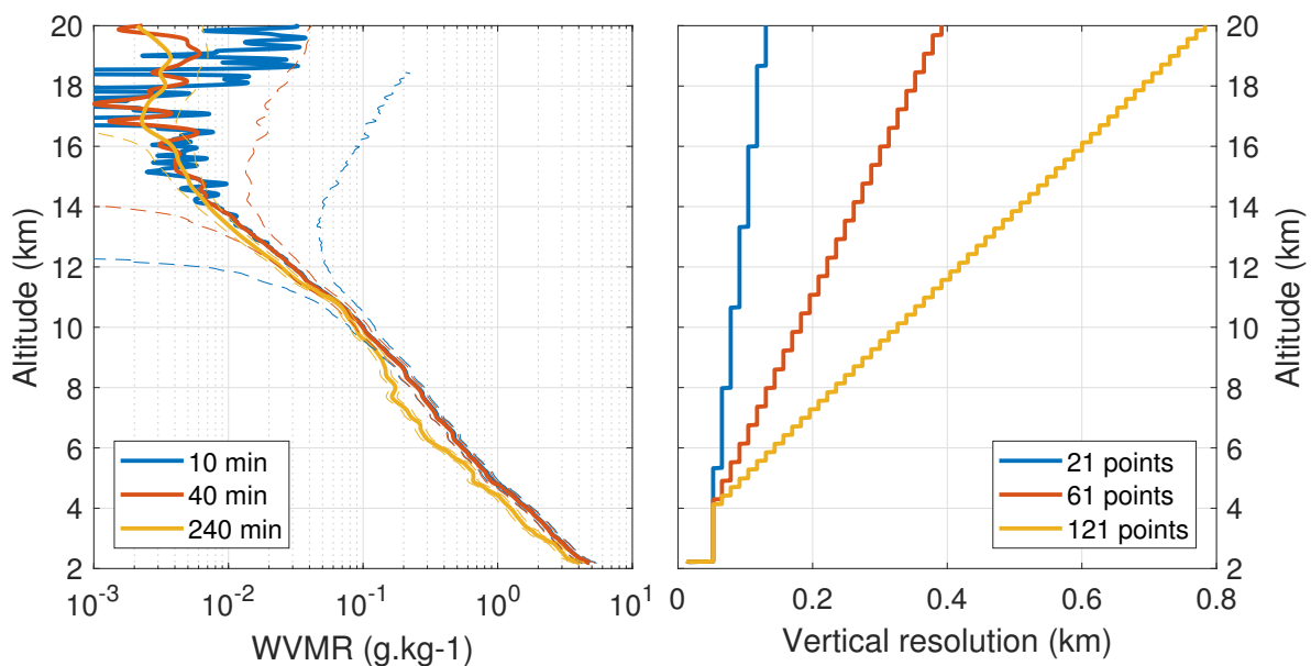
Figure 4. Mean profiles integrated over 10 min (solid blue line), 40 min (solid orange line) and 240 min (solid yellow line) with their total uncertainty (dotted lines) ( left ), and the associated vertical resolution ( right ) according to the altitude above sea level.
