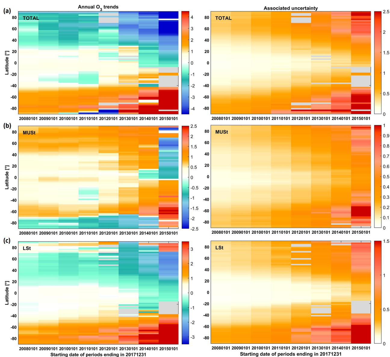
Figure 12. Evolution of estimated linear trend ( \text{DU yr}^{-1} ) and associated uncertainty accounting for the autocorrelation in the noise residuals ( \text{DU yr}^{-1} ; within the 95 % confidence level) in (a) total, (b) MUST and (c) LSt O 3 columns, as a function of the covered IASI measurement period ending in December 2017, with all natural contributions estimated from the whole IASI period (2008–2017; date format in the figure is yyyyddmm). Note that the scales are different between the columns.
