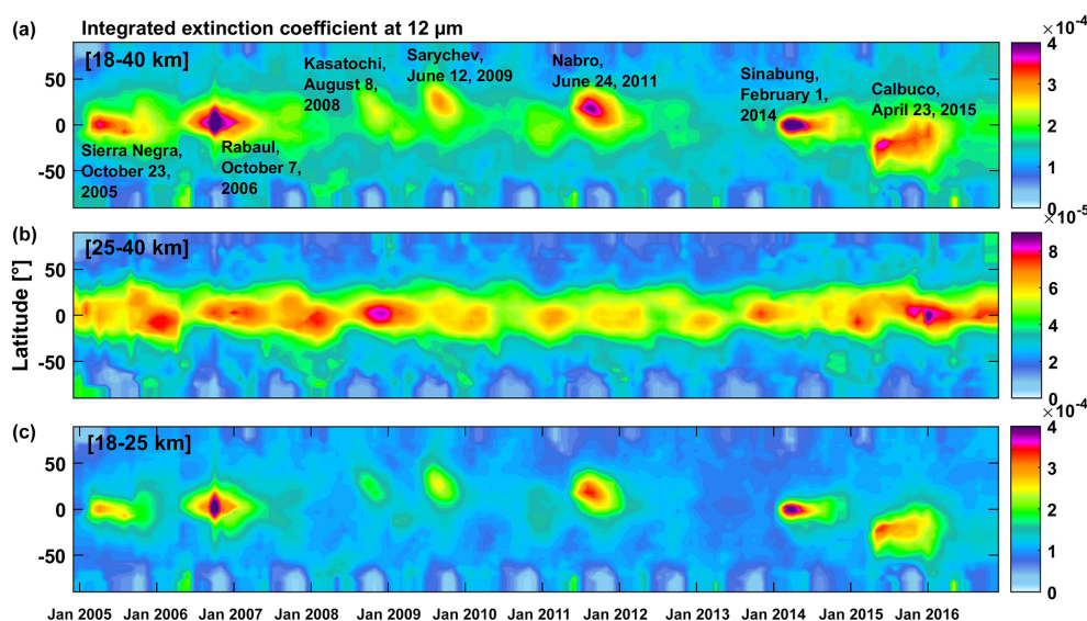
Figure 3. Latitudinal distribution of volcanic sulfuric acid extinction coefficient at 12\ \mu\text{m} integrated (a) over the stratosphere, (b) over the middle stratosphere and (c) over the lower stratosphere, as a function of time from 2005 to 2017. The dataset consists of monthly mean aerosol data merged from SAGE, SAM, CALIPSO, OSIRIS, 2-D model simulation and Photometer (processed at NASA Langley Research Center, USA, and ETH Zurich, Switzerland).
