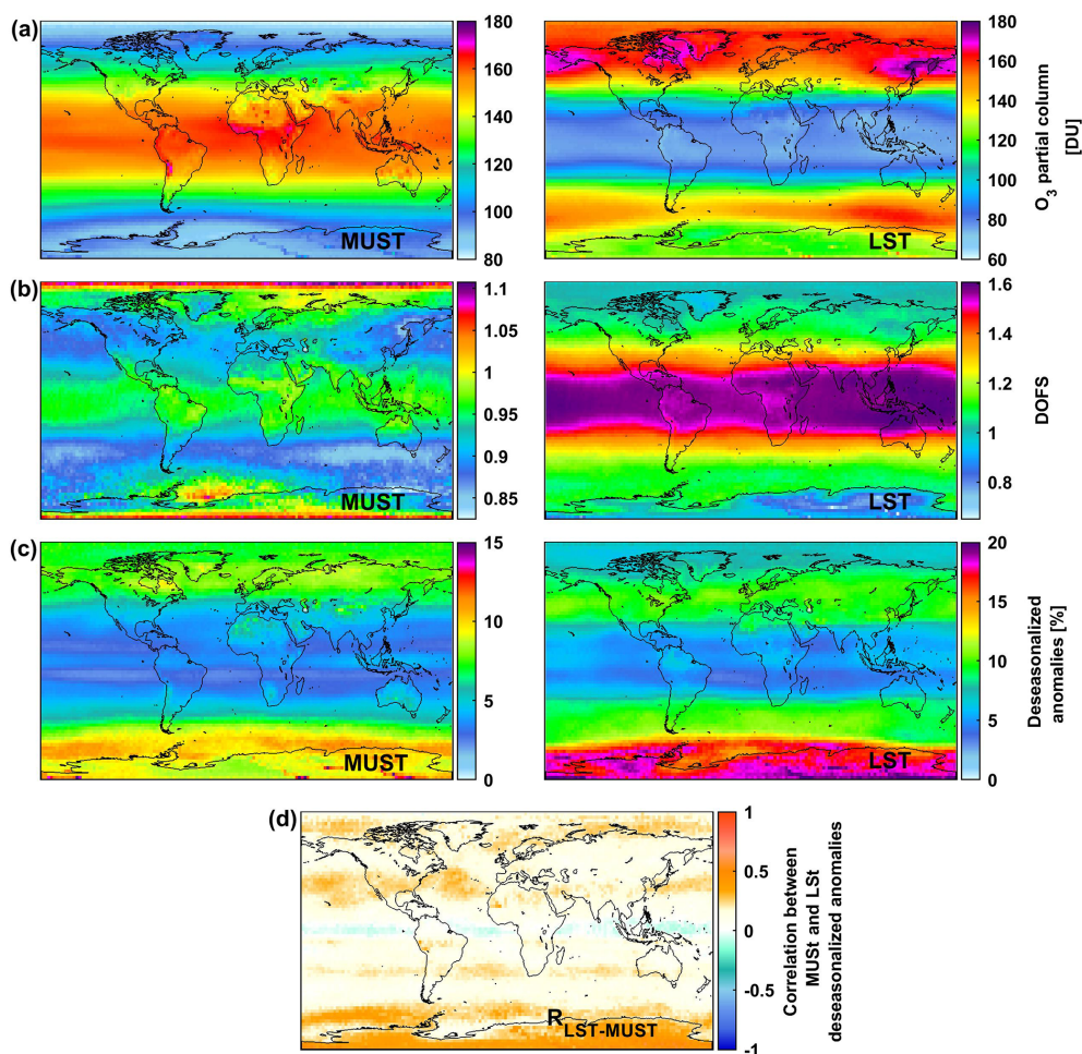
Figure 1. Global distribution of (a) daily O 3 columns (in Dobson units – DU), (b) associated DOFS, (c) absolute deseasonalized anomalies (in percentage) averaged over January 2008–December 2017 in the MUST (middle–upper stratosphere: > 25 hPa; left panels) and in the LSt (lower stratosphere: 150–25 hPa; right panels). Panel (d) shows the correlation coefficients between the daily O 3 deseasonalized anomalies in the MUST and in the LSt. Note that the scales are different between MUST and LSt.
