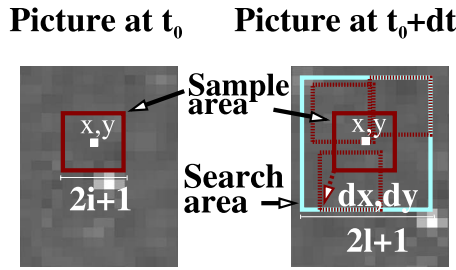
FIG. 2. (Color online) For the CIV technique the gray-level of two pictures in a time sequence is compared. In red (dark gray) a sample area is defined in the first picture. In the following picture it is then tried to find a similar area with the same gray-level distribution within the search area shown in blue (light gray).
