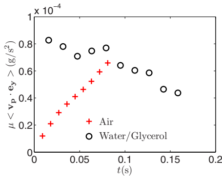
FIG. 18. (Color online) The velocity y component multiplied by the fluid viscosity averaged over the first ten lowest particles in time.
