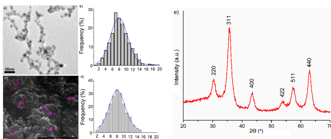
Figure 6. Large-area TEM (a), size distributions from TEM (b), SEM image (c) and size distributions from SEM (d) of iron oxide coated with dextran and X-ray diffraction pattern of dextran-coated maghemite nanoparticle (D-MNPs) (e).
