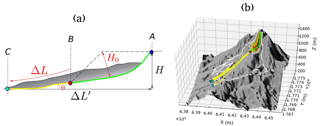
Figure 10. Computation of \mu_H and \mu_{eff} . (a) Landslides metrics in 2D (after 52 ). A (blue point) and B (red point) are respectively the highest and the lowest points of the initial mass. C (cyan point) is the flow front position. H_0 is the initial mass maximum thickness. H and \Delta L' are respectively the difference in altitude and horizontal distance between A and C. \Delta L is the length traveled by the front flow, i.e. the length of the yellow curve. \theta is the mean local slope between A and C, i.e. the mean local slope of the joint yellow and green curves. The Heim's ratio is \mu_H = H/\Delta L' , and the effective friction coefficient is \mu_{eff} = \tan(\theta) + H_0/\Delta L . (b) Landslides metrics in 3D, for the topA2 scenario with \delta = 10 . Color code of lines and points matches (a) . The white line is the deposit extent, the dashed white line is the collapse scar extent. Colorscale in the collapse geometry matches the initial mass thickness (from yellow to red). Points A and B are uniquely defined. Points C are chosen as explained in the main body of the text. The DEM is from IGN BDTopo, coordinates: WGS84, UTM20N.
