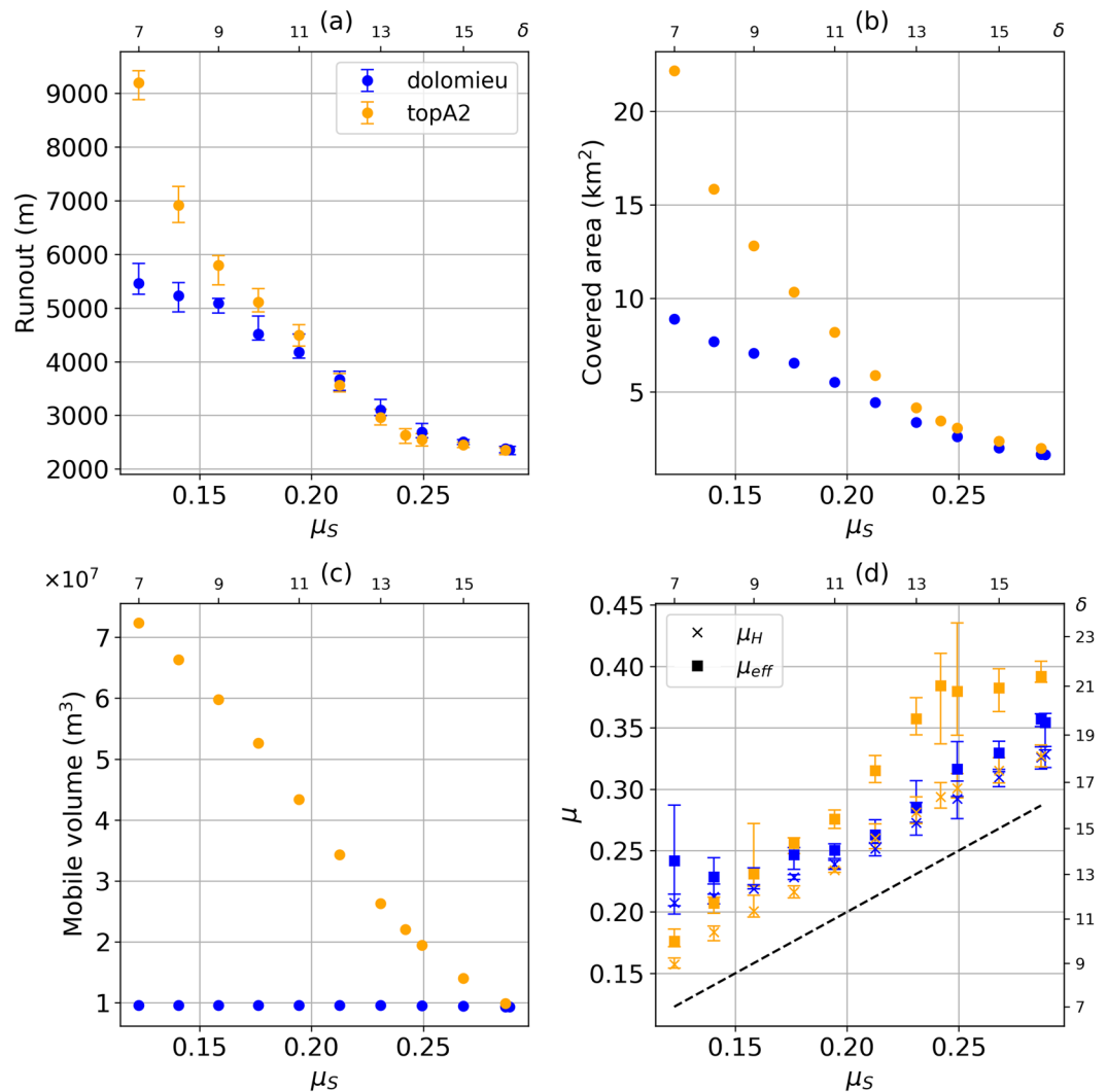
Figure 9. Main characteristics of debris avalanche deposits for the dolomieu (blue) and topA2 (orange) scenarios. Varying friction coefficient are tested (from \delta=7^\circ to \delta=16^\circ ). (a) Runout, i.e. maximum distance between the highest point in the collapse structure prior to collapse and flow front. (b) Covered area. (c) Mobile volume, i.e. volume of the material leaving the collapse structure (d) Heim's ratio (crosses) and effective friction coefficient (squares). Values on the right y-axis in (d) and top x-axis are the angles \delta in degrees, matching \mu on the opposite axis, such that \mu = \tan(\delta) . Error bars in (a) and (d) display the maximum, minimum and mean value derived following the methodology presented in the body of the text.
