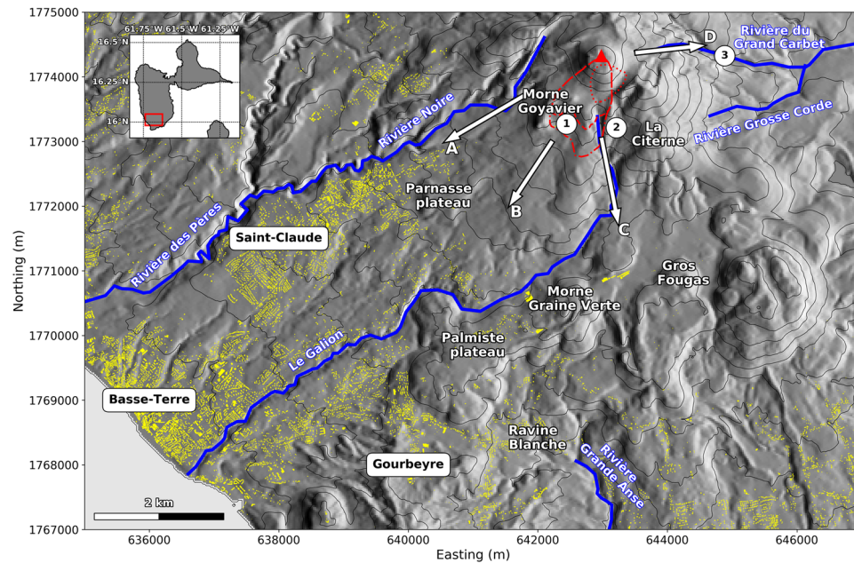
Figure 1. Rivers and main topographic features around La Soufrière de Guadeloupe volcano (red triangle), along with the three main cities (Saint-Claude, Basse-Terre and Gourbeyre). The upper left inset features the Guadeloupe island, with the red rectangle matching the extent of the map. ① Ravine des Bains Jaunes, ② Ravine de la Citerne, ③ Second Carbet waterfall. Arrows A, B, C and D identify the main flow pathways discussed in the main body of the text. Yellow patches are buildings (data from IGN BDAlti). The lateral extent of some initial unstable volumes is displayed with the red lines. Dashed-dotted line: topA2 and midA2 scenarii; dashed line: topA1_inf and topA1_sup scenarii; dotted line: dolomieu scenario. The DEM is from IGN BDTopo, coordinates: WGS84, UTM20N. The contour interval is 100 m.
