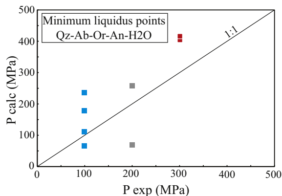
Fig. 5. Comparison between experimental ( P_{\text{exp}} ) and calculated ( P_{\text{calc}} ) pressures for minimum liquidus points in the \text{Qz}–\text{Ab}–\text{Or}–\text{An}–\text{H}_2\text{O} system, both An-free and An-bearing. The calculated pressures are obtained with the DERP geobarometer (Wilke et al., 2017). Experimental and calculated pressures are from Table 2. Experimental data points for each pressure are distinguished using the same color code as in Fig. 3.
