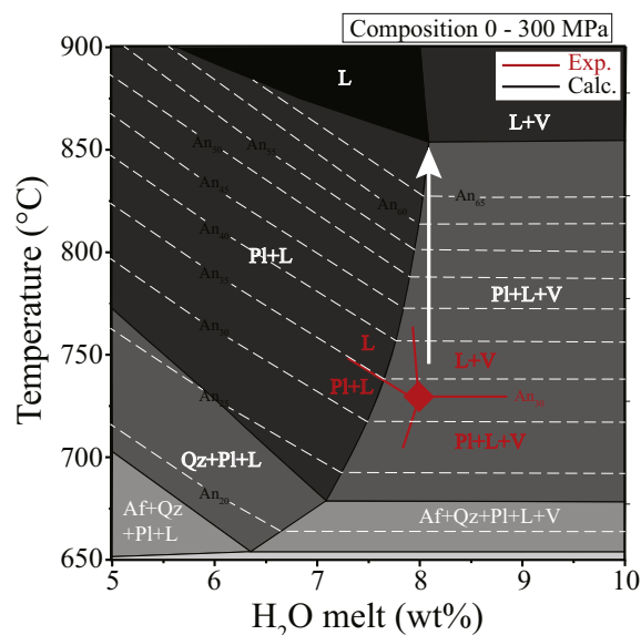
Fig. 6. Experimental and calculated phase equilibria for composition 0 (Table s1) at 300 MPa projected on a temperature (°C) vs. \text{H}_2\text{O} concentration in melt (wt%) diagram. Abbreviations: L, liquid; V, fluid phase; Af, alkali feldspar; Pl, plagioclase; Qz, quartz; An, 100 \text{Ca}/(\text{Ca} + \text{Na}) in plagioclase. Calculated data are shown in black, white and grey, and experimental data in red. The calculated stability fields, phase assemblages and compositions are obtained with the model of Holland and Powell (2001). Dashed lines indicate plagioclase An contents. The large red diamond is the \text{H}_2\text{O} -saturated experimental temperature (plagioclase saturation) point (Table 1). Notice the marked differences between the calculated (860 °C) and the experimental (730 °C) temperature of the \text{H}_2\text{O} -saturated plagioclase saturation point and between the calculated (>65) and experimental (30) An content of the liquidus plagioclase.
