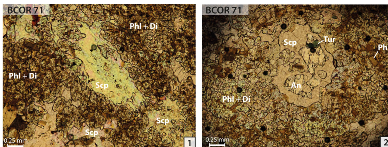
Fig. 4. Thin-section micrographs showing the main features of Type I samples: (1) “micaceous hornfels” clast. Note the poikiloblastic texture of the central scapolite, with numerous inclusions (plane-polarized light; sample BCOR 71); (2) “Micaceous hornfels” clast. Note the tourmaline and anorthite inclusions in the central scapolite (plane-polarized light; sample BCOR 71). Abbreviations from Whitney and Evans (2010) .
