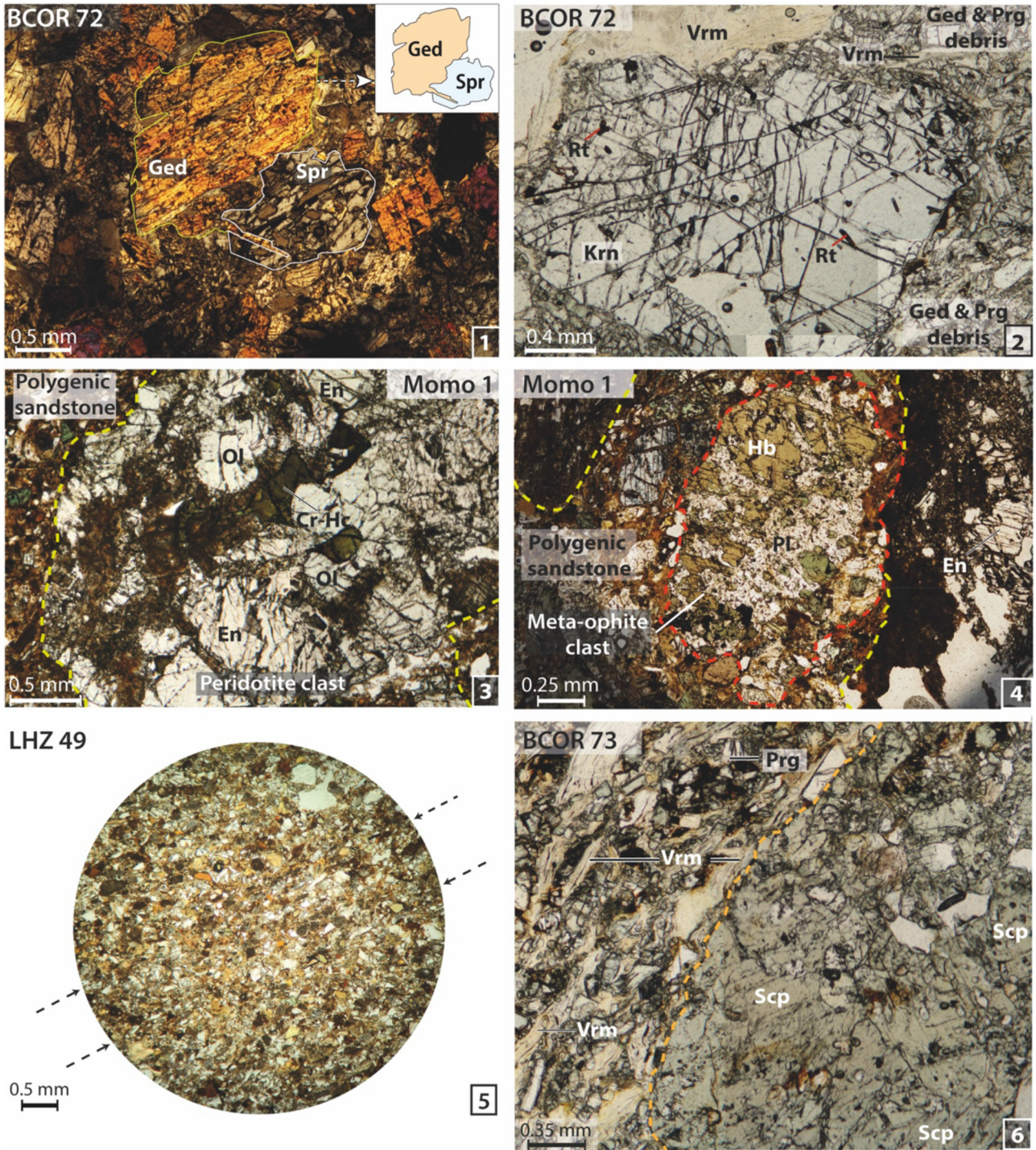
Fig. 6. Representative micrographs of Type III samples: (1) polymineralic clast of sapphirine + gedrite showing textural equilibrium between the two phases (redrawn in the inset; cross-polarized light; sample BCOR 72). Areas appearing in brown in the sapphirine crystal correspond to voids generated when the thin section was prepared; (2) millimetric subhedral kornierupine crystal displaying parallel-oriented rutile inclusions (plane-polarized light; sample BCOR 72); (3) peridotite clast. Yellow dotted lines underline the limits of the polymineralic clast (plane-polarized light; sample Momo 1); (4) meta-ophite clast underlined by a red dotted line. Two ultramafic clasts are underlined by yellow dotted lines (plane-polarized light; sample Momo 1); (5) polymictic sandstone exclusively made of monomineralic clasts. A coarse bedding is underlined by planar minerals (black dotted arrows parallel to the bedding; plane-polarized light; sample LHZ 49); (6) polymineralic clast of scapolite (underlined by an orange dotted line) enclosed in a sandstone made of monomineralic clasts. Note the orientation of the vermiculite flakes, parallel to the borders of the scapolite clast (plane-polarized light; sample BCOR 73). Abbreviations from Whitney and Evans (2010) .
