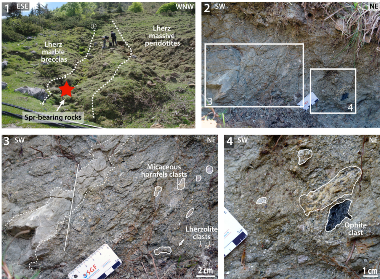
Fig. 3. Field photographs from site 2: (1) photograph of the contact zone between the mantle peridotites and the Lherz breccias at site 2 and location of the sapphire-bearing rocks sampling site (red star). White dotted lines underline the progressive transition existing between the Lherz body and the Lherz marble breccias. Around white dotted line n° 1, a progressive transition from the sapphire-bearing rocks to the pure marble breccias and microbreccias was observed; (2) detailed view of the sampling site 2 and location of close up photographs 3 and 4 shown below; (3) detailed view of the left side of exposure. It consists of a pale-green to light-grey microbreccia showing a rough bedding with layers of thin-grained sandstones dipping to the south-east (dashed lines). The microbreccia contains numerous cm-sized angular clasts of variable lithologies including “micaceous hornfels” and poorly serpentinized lherzolite (white outlines, determined on thin-sections); (4) detailed view of the right side of exposure. Sandstones include numerous cm-sized angular clasts of variable compositions (white outlines). One black clast of meta-ophite is observed macroscopically (bottom right side of photograph).
