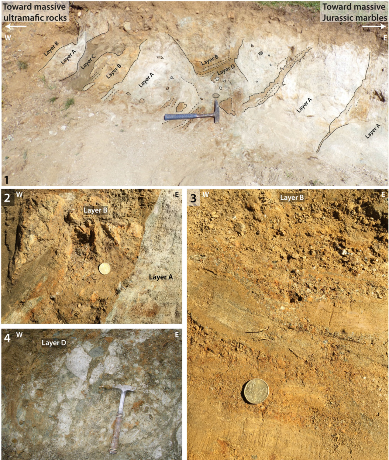
Fig. 2. Field photographs from site 1: (1) succession of clastic layers at site 1. Four layer types can be distinguished (see text for complete description). The dominant Layer A corresponds to light grey, coarse sandstones. Layer B corresponds to dark-brown layers of ultramafic breccias and microbreccias composed of dominant angular clasts of serpentinized lherzolite in an ultramafic sandy matrix. Layer C is represented by breccias and sandstones made of dominant ultramafic and minor cm-sized clasts of Triassic meta-ophite. Layer D is a coarse breccia composed of cm- to dm-sized angular clasts of ultramafic rock, white microbreccias, Triassic to Lower Jurassic meta-ophites and “micaceous hornfels”; (2) sharp contact between Layer B ultramafic breccias (left) and light-grey Layer A sandstones (right); (3) close-up of graded-bedding observed in Layer B microbreccias; (4) detail view of Layer D breccia.
