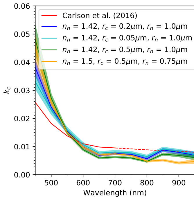
Figure 9: Chromophore imaginary refractive index solutions k_c(\lambda) retrieved through limb-darkening analysis of the NEB (showing the four solutions with the best \chi^2/n values) compared with the tabulated optical constants of Carlson et al. (2016), with the legend as in Figure 7 with uncertainties shaded. We can see that the general shape of the retrieved solutions of k_c(\lambda) is relatively invariant regardless of r_c , with only minor modifications needed to the spectral slope.
