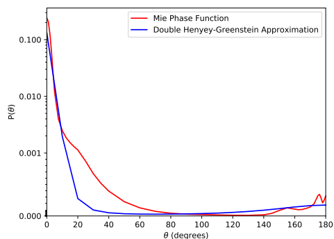
Figure 5: Example normalised Mie phase function (for a conservatively-scattering particle of radius 4\mu\text{m} ) at a wavelength of 700\text{ nm} , compared to the equivalent ‘smoothed’ phase function computed using the double Henyey-Greenstein approximation.
