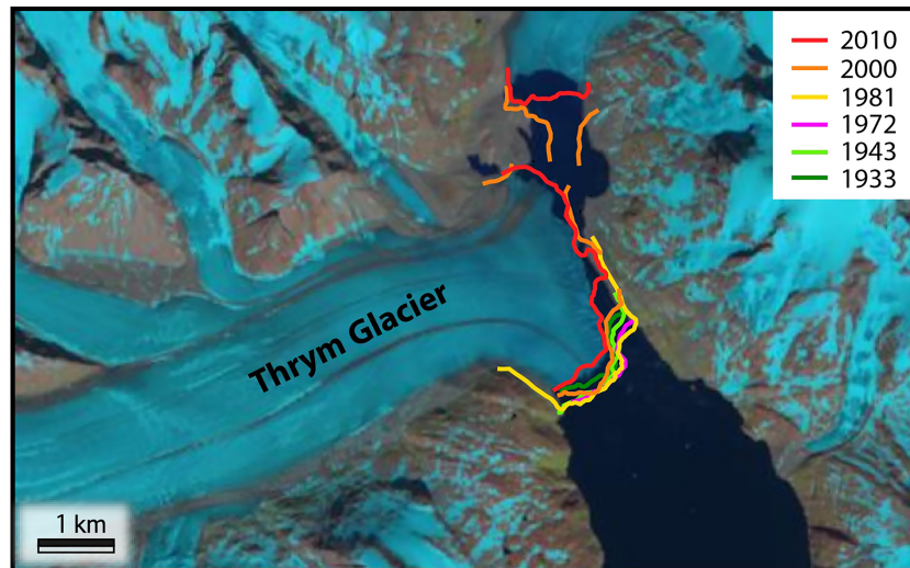
Figure 2. Landsat Satellite image of Thrym Glacier (June 2014) with observed terminus positions since 1933.
