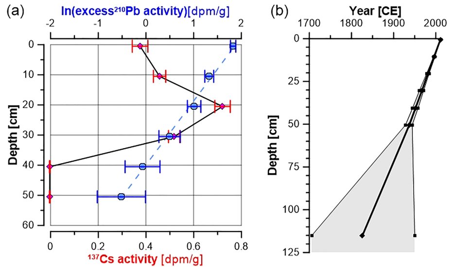
Figure 4. (a) Downcore profile of activity in excess ^{210}\text{Pb} (blue) shown on a logarithmic scale versus depth. ^{137}\text{Cs} activity is in red. (b) Results of dating versus depth, with the oldest/youngest calibrated ages in thin line and the average indicated by the thick line.
