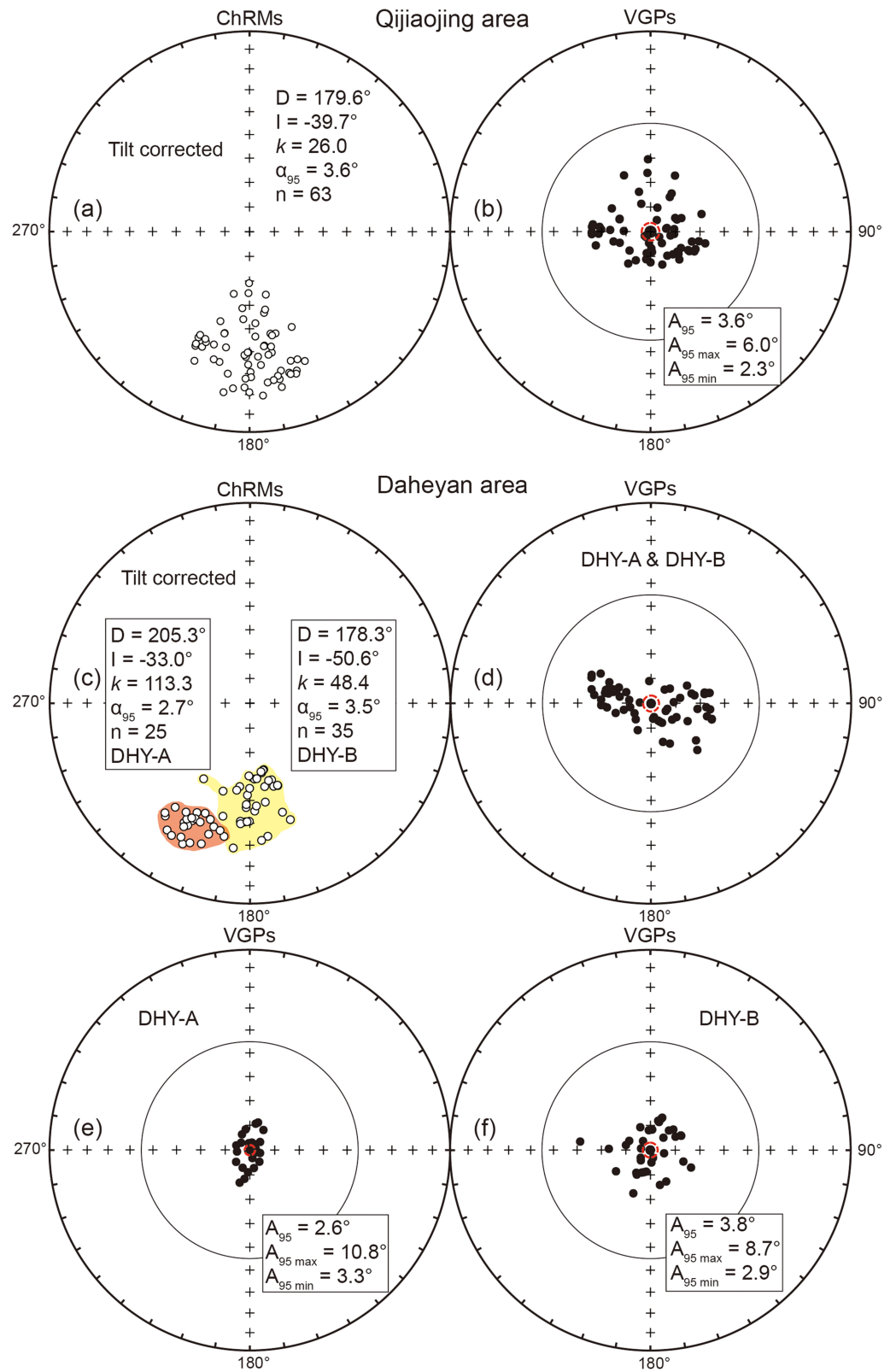
Figure 7. Equal-area projections of the isolated ChRM directions in stratigraphic coordinates from the Qijiaoqing section (a) and Daheyan (DHY-A and DHY-B) section (c) and the corresponding VGPs for the Qijiaoqing section (b), Daheyan (DHY-A & DHY-B) section (d), DHY-A section (e), and DHY-B section (f). Cutoff criterion of 45° is used after Deenen et al. (2011).
