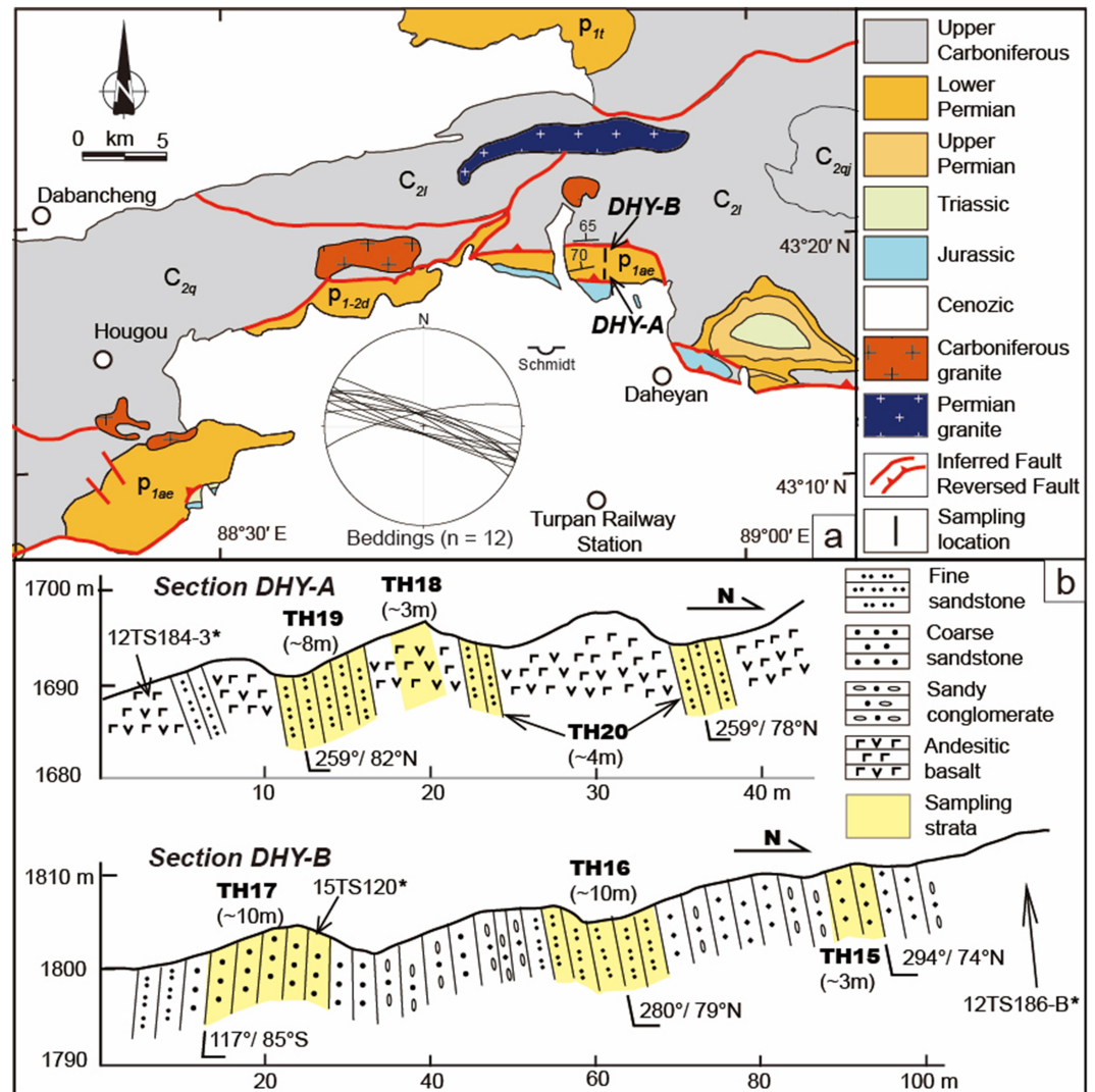
Figure 3. (a) Geologic map of the Daheyan area, NW of the Turpan-Hami Basin (modified from XBGMR, 1960, 1988 and XGSC, 2007). DHY-A and DHY-B stand for two sampled sections. (b) Cross sections of two studied sections in the Daheyan area. stratigraphic positions of paleomagnetic sampling sites and geochronological samples are shown. Note that geochronological samples labeled with * are after Wali et al. (2018). DHY = Daheyan.
