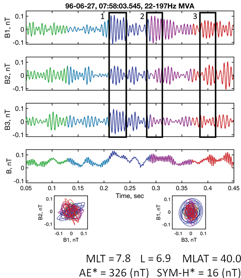
Figure 3. A \sim 0.4 s interval with a variety of wave polarizations. Five different colorizations with equal time intervals have been used to allow the reader to follow the evolution of the waves. The top four plots are the magnetic field components in minimum variance coordinates and the wave magnetic field magnitude variations. The bottom two plots are the B1-B2 and B3-B1 hodograms. The event occurred on June 27, 1996.
