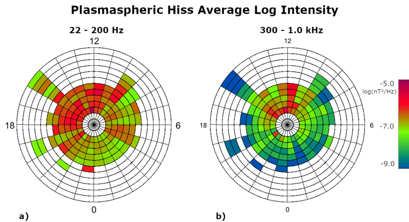
Figure 1. A comparison of the intensity and location of LF plasmaspheric hiss ( \sim 22 to 200 Hz), panel a), to HF plasmaspheric hiss ( \sim 300 Hz to 1.0 kHz), panel b) for the 1-year Polar study. For both panels, noon is on the top, and dusk is on the left. The coverage extends from L = 2 to L = 13 . The legend on the right gives the average of the log intensities of 2 min intervals for each \Delta L - \Delta MLT bin. The bin size is 1 hr MLT and 1 L shell. Panel (b) was taken from Tsurutani et al. (2018).
