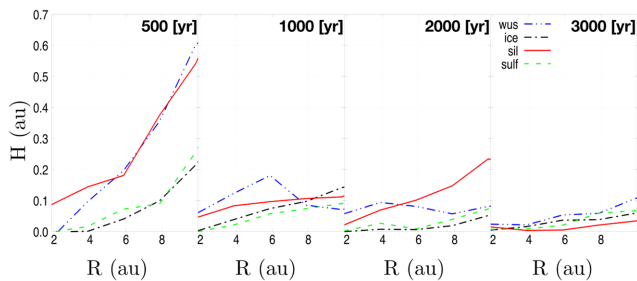
Figure 2. Scale height H for different species at the selected time. Ice and sulphides settle more efficiently when compared with wustite and silicates. This is due to the different fragmentation thresholds that make the growth and, thus, the settling of wustite and silicate less efficient. This behaviour is opposite to that found when only pure growth is taken into account.
