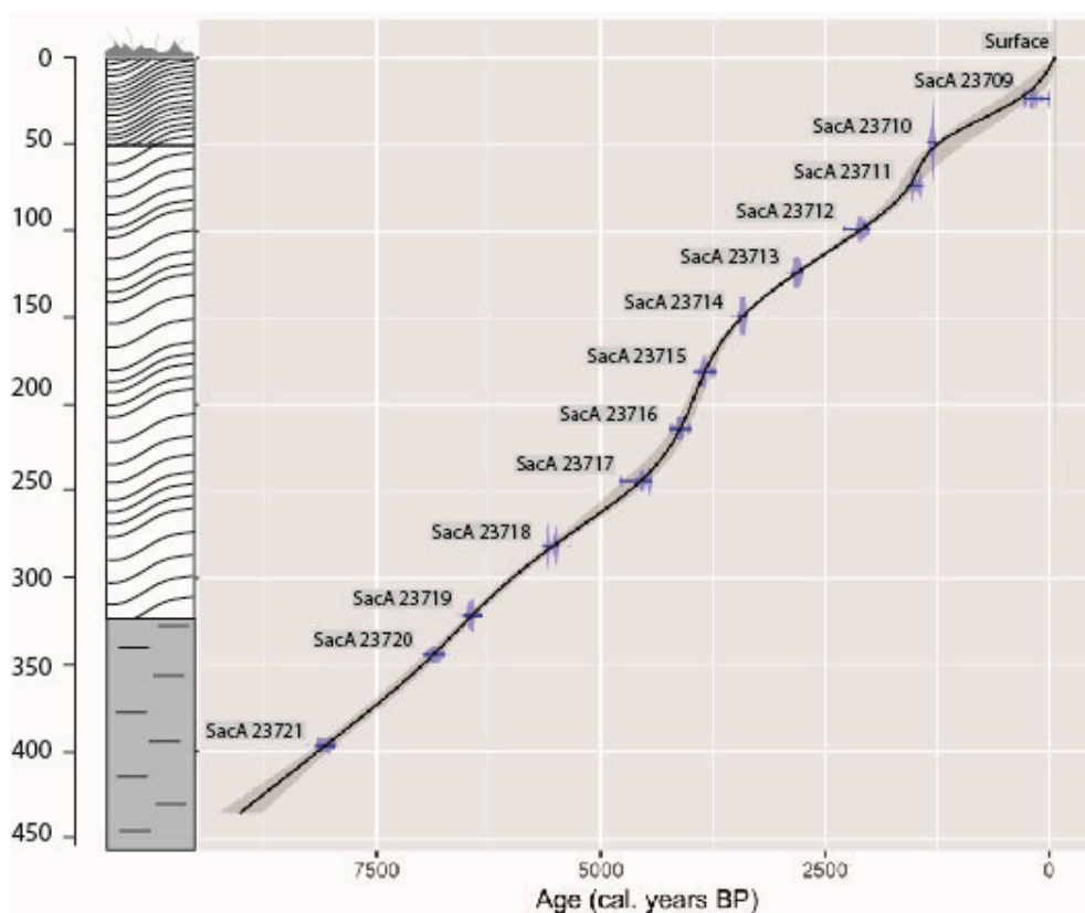
Figure 2. Peat core stratigraphy (1: clay; 2: successive layers of sapric and fibric peat; 3: compact and fibrous peat) and age–depth model, using a smooth polar interpolation of 13 radiocarbon dates.
