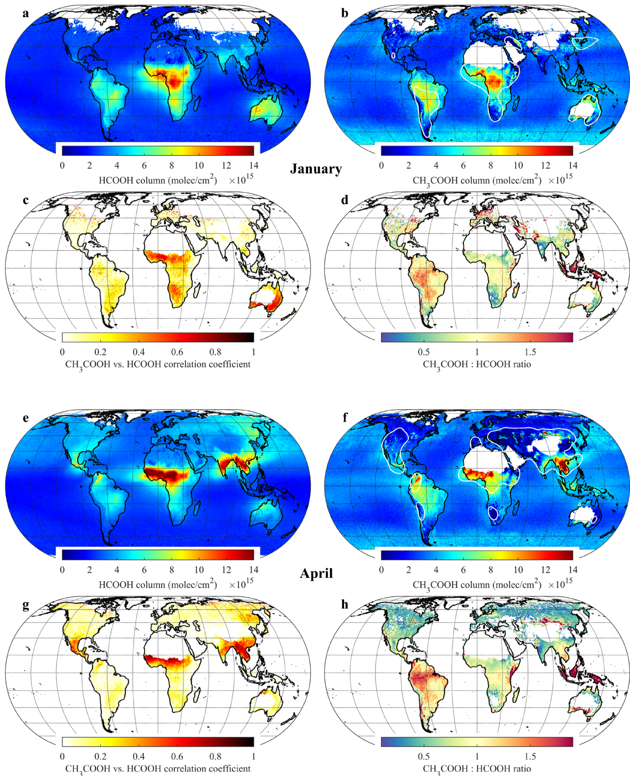
Figure 2. (a–b) Means (on a 0.5^\circ \times 0.5^\circ grid) of the HCOOH and \text{CH}_3\text{COOH} total columns from the 2007–2018 IASI/Metop–A observations over January. The empty spaces at high latitudes are regions where no measurements passed the pre- and post-filtering. The \text{CH}_3\text{COOH} data over deserts are not displayed. The white contour lines delimit the areas with high \text{CH}_3\text{COOH} measurement confidence (see text). (c) Correlation coefficients between the daily 0.5^\circ \times 0.5^\circ gridded HCOOH and \text{CH}_3\text{COOH} total columns and (d) \text{CH}_3\text{COOH}:\text{HCOOH} column ratios, over January throughout the 2007–2018 time period. (e–h) Same as (a–d), but for April.
